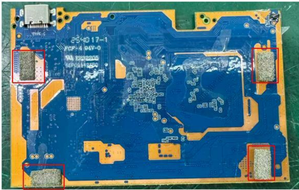
Conductive sponge is attached to the exposed copper area at the bottom of the motherboard
