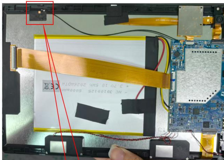
WiFi天线
