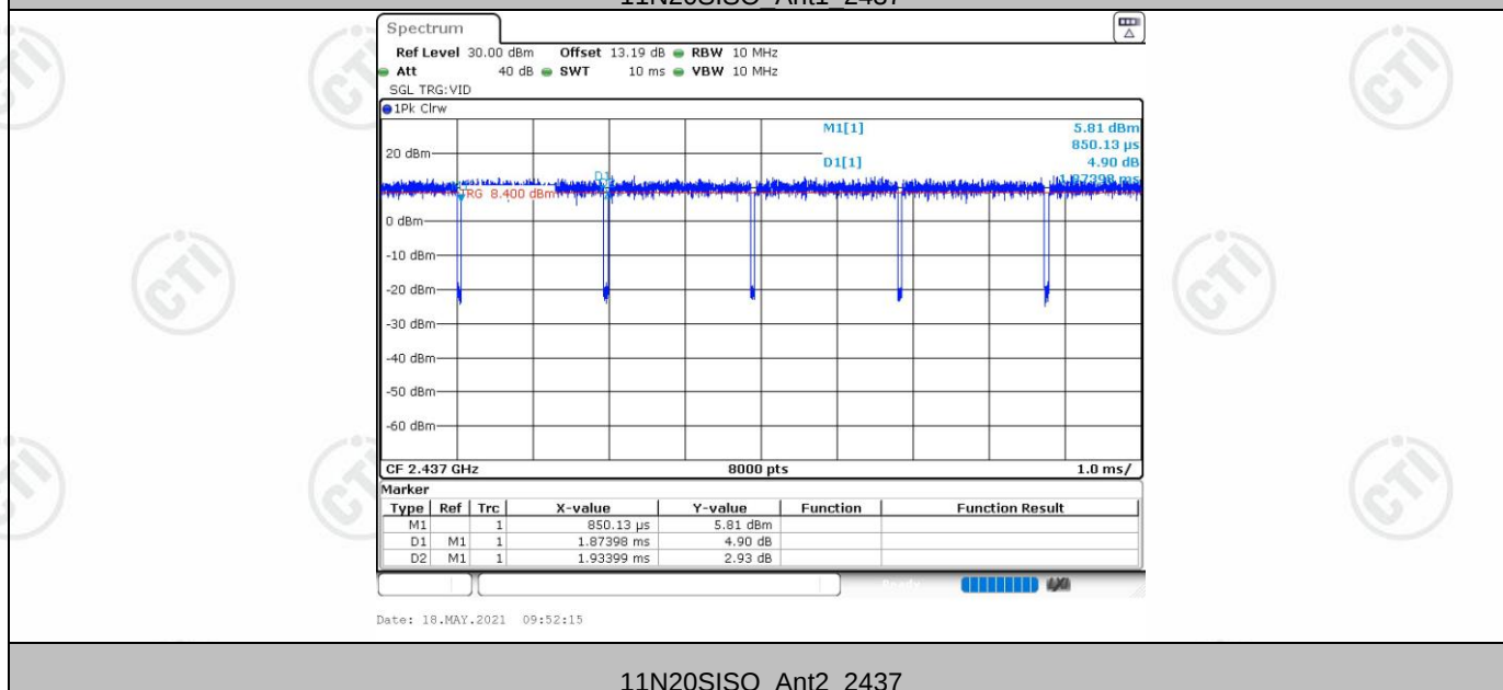
11N20SISO Ant1 2437
