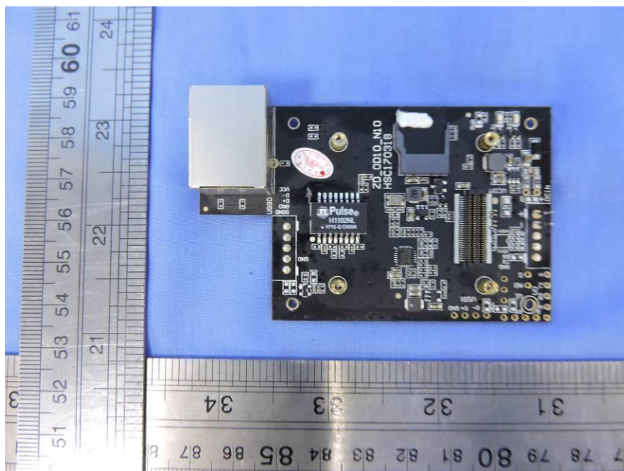
Camera Bottom Board(Front)
