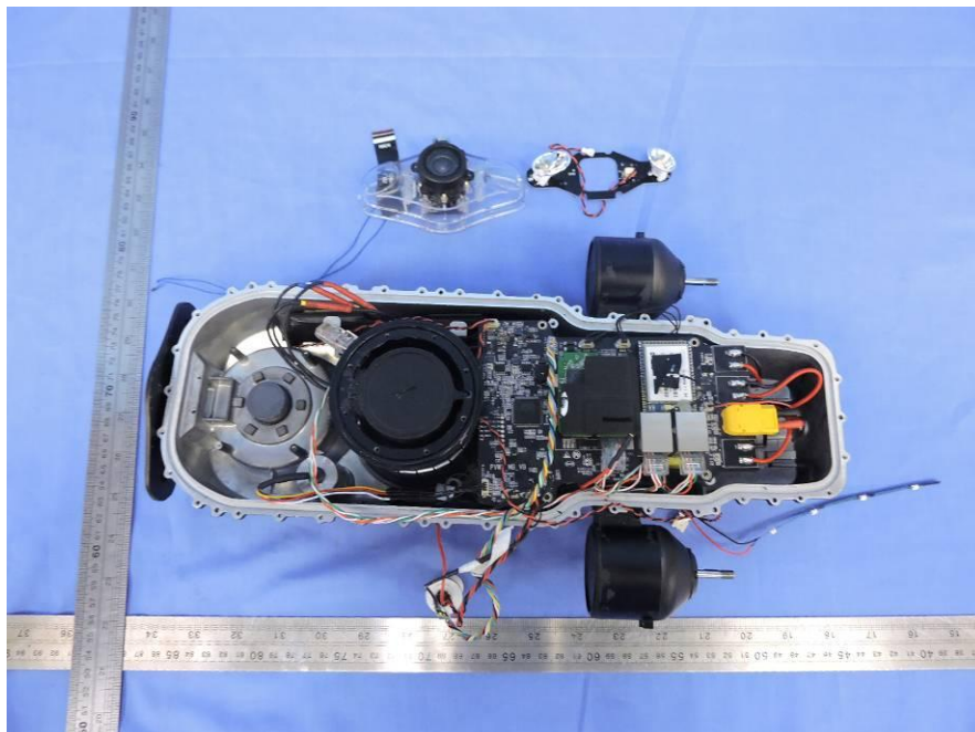
Camera Core Board (Back)
