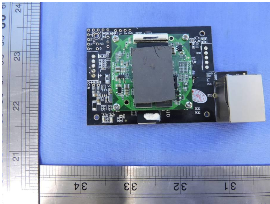
Camera Board
