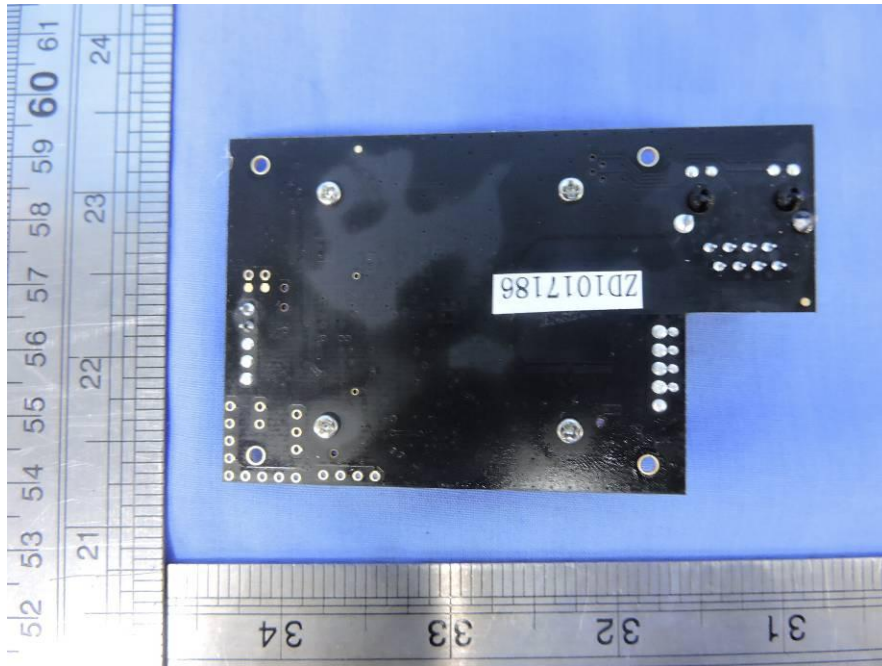
Camera Bottom Board(Back)
