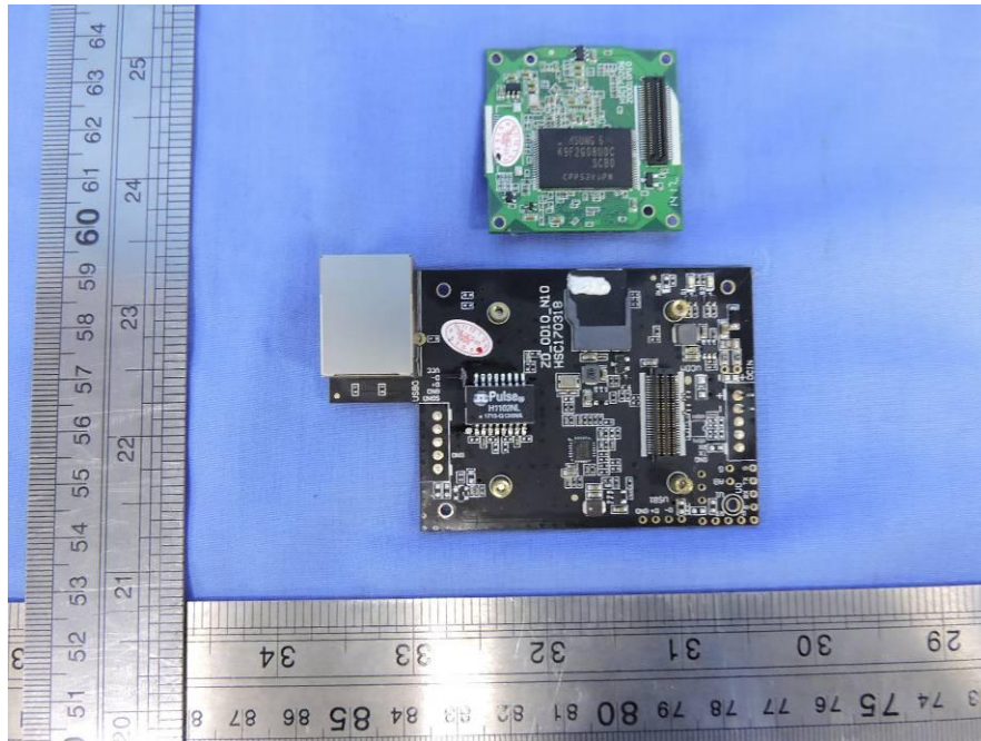
Camera Core and Bottom Board
