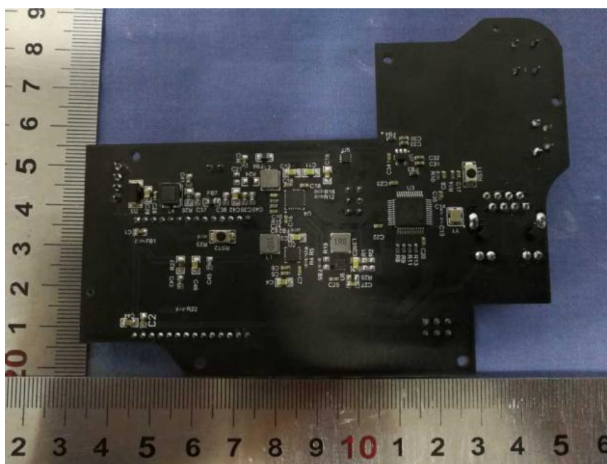
Base board(Back)
