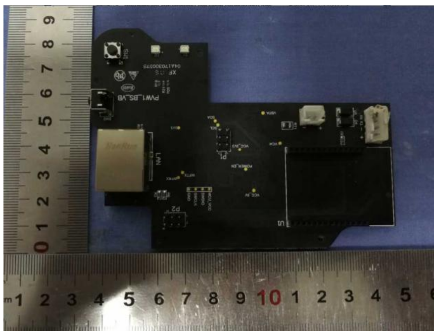
Base board(Front)
