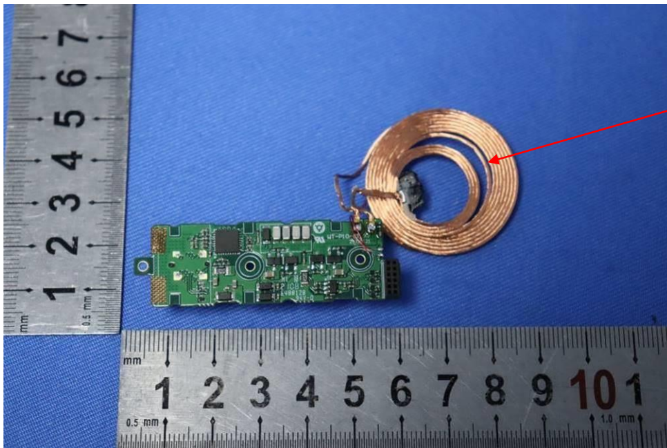
WPC antenna
