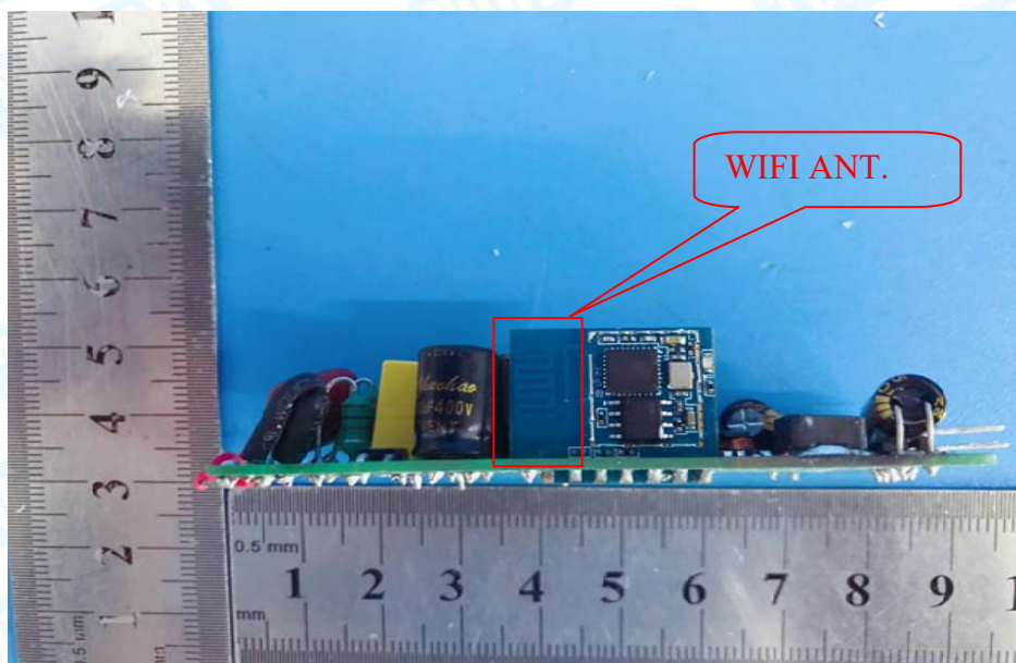
Photo 10 Appearance of PCB
