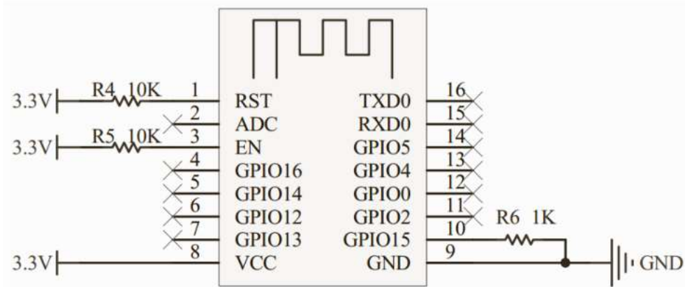
Figure -6. ESP8266-12H minimum system
