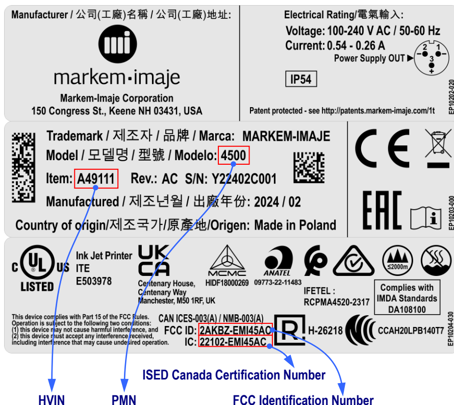
Fig. 2. Model 4500 - three-label manufacturer's nameplate located on the side of the power supply module
