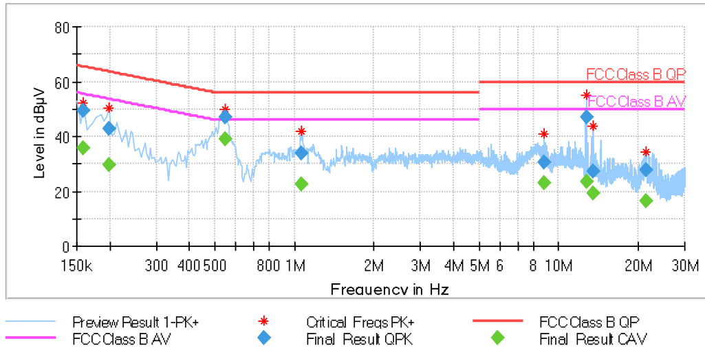
Full Spectrum
