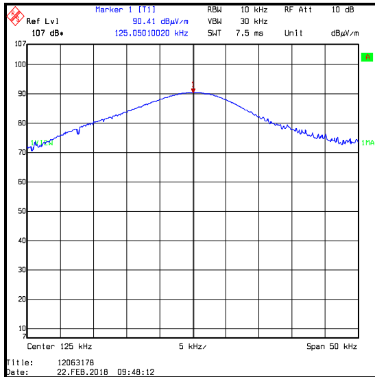
125 kHz reference unit signal at 3 metres on an open field test site on 22 February 2018
