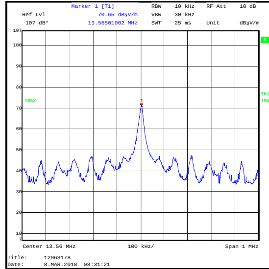
13.56 MHz reference unit signal at 3 metres in a semi-anechoic chamber on 08 March 2018
