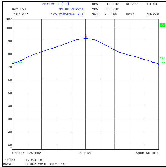
125 kHz reference unit signal at 3 metres in a semi-anechoic chamber on 08 March 2018
