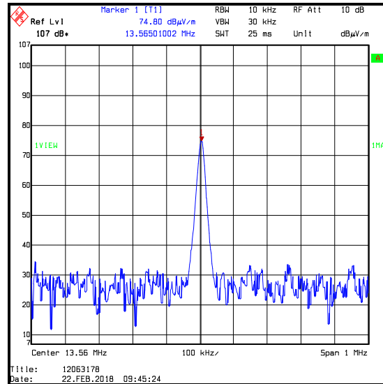
13.56 MHz reference unit signal at 3 metres on an open field test site on 22 February 2018
