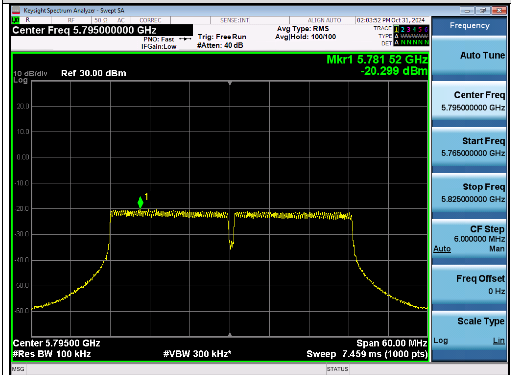
Test_Graph_802.11n40_ANT1_5795_MCS0_PSD
