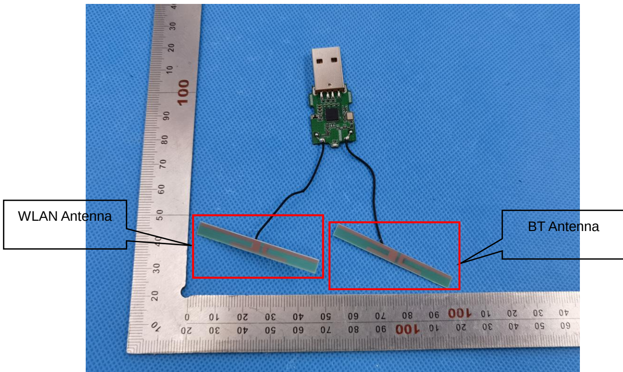
INTERNAL VIEW OF EUT (FIGURE 4)
