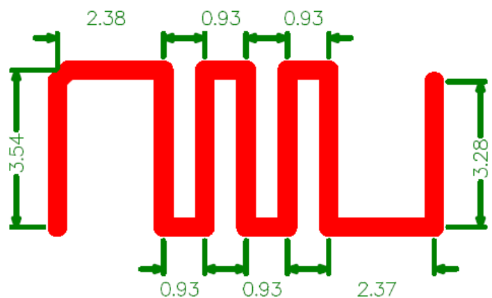
Antenna Layout and Size
