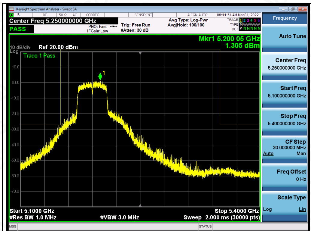
Test_Graph_802.11n40_ANT1_5190_MCS0_Frequency Band 3
