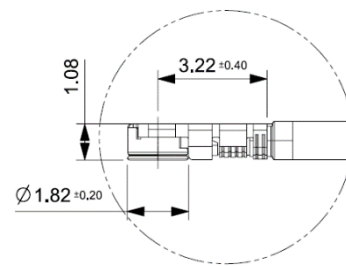
DETAIL B SCALE 8:1 CONNCECTOR
