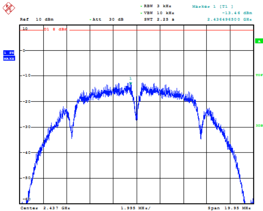
PSD-Pk-Ch6-bMode-1Mbit
