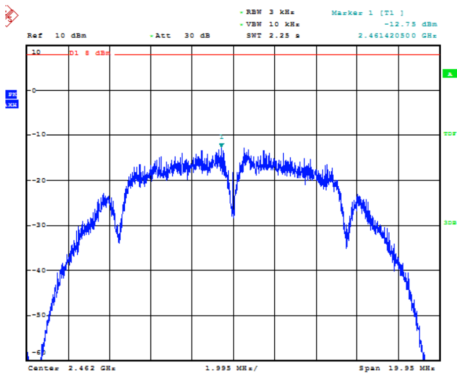
PSD-Pk-Ch11-bMode-1Mbit
