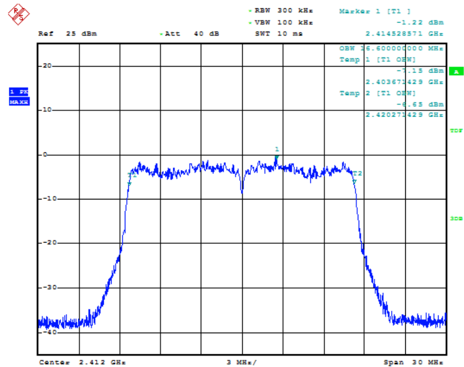
99%-BW-Ch1-gMode-24Mbit
