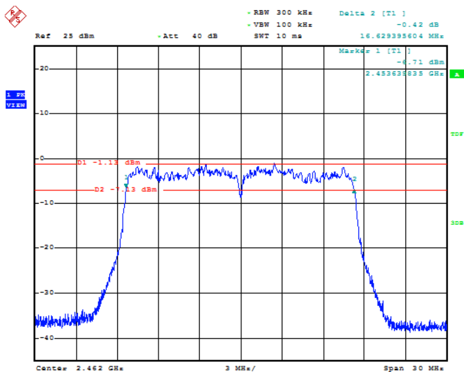
6dB-BW-Ch11-gMode-24Mbit
