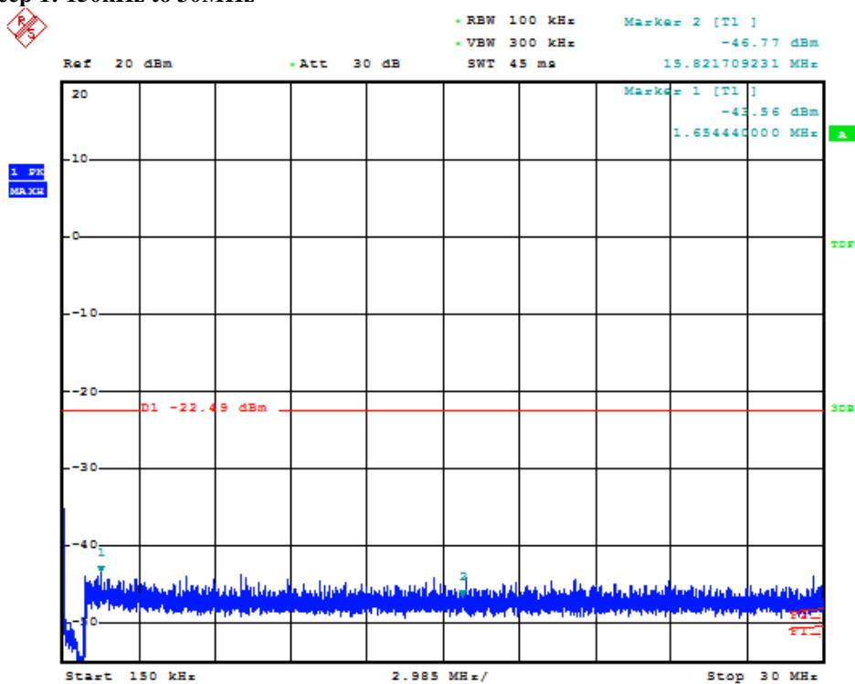
20dBc-0.15-30MHz--Ch11-gMode-24MBit
