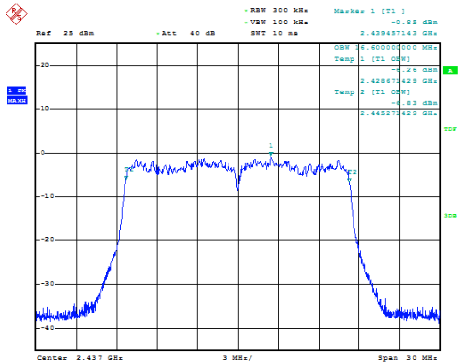
99%-BW-Ch6-gMode-24Mbit
