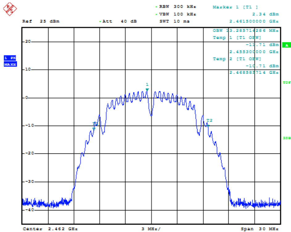
99%-BW-Ch11-bMode-1Mbit
