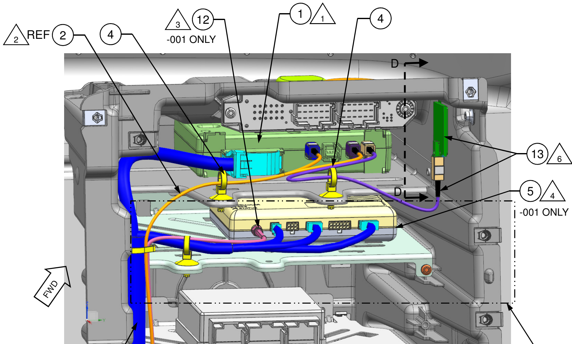
VIEW C ECU INSTALLATION (FROM PAGE1)
