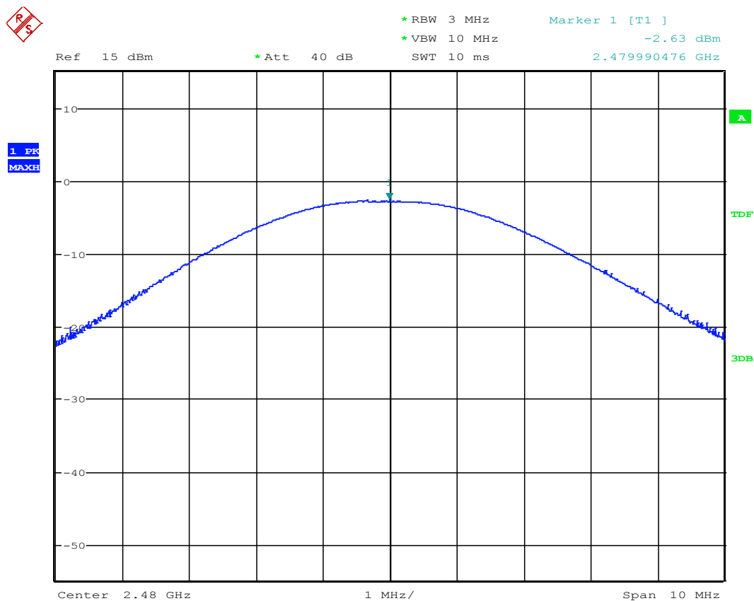
Peak Power_high_2480
