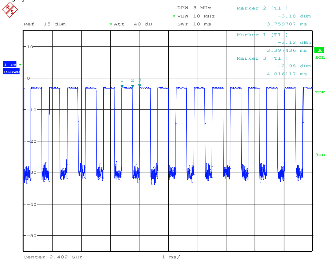
DC_low_2402
