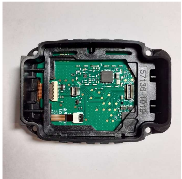
Fig 2. Prism V2 Capsule Upper Board
