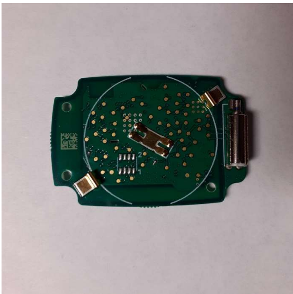
Fig 3. Prism V2 Main Board Battery side
