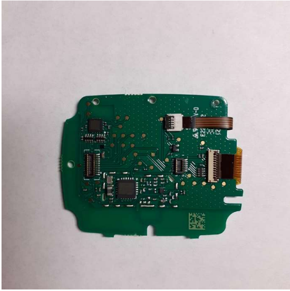
Fig 5. Prism V2 Upper Board Component side
