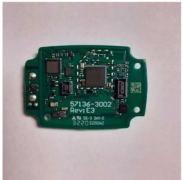
Fig 4. Prism V2 Main Board Component side
