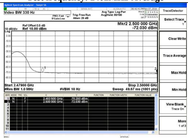
Test frequency: 2480MHz-Average
