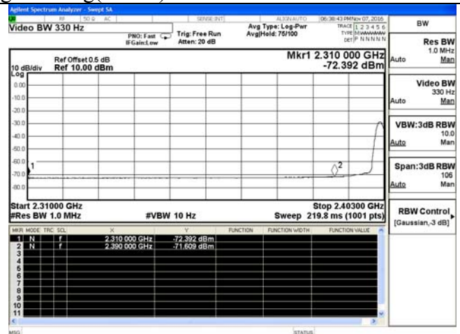
Test frequency: 2402MHz-Average
