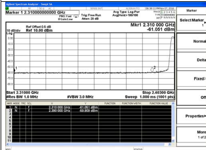
Test frequency: 2402MHz-Peak
