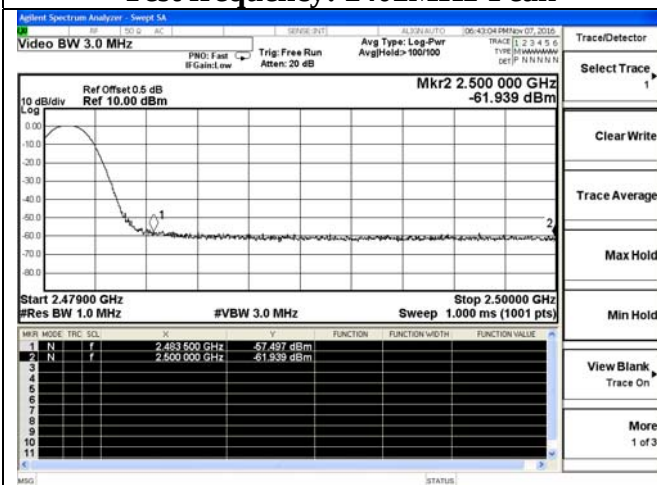
Test frequency: 2480MHz-Peak
