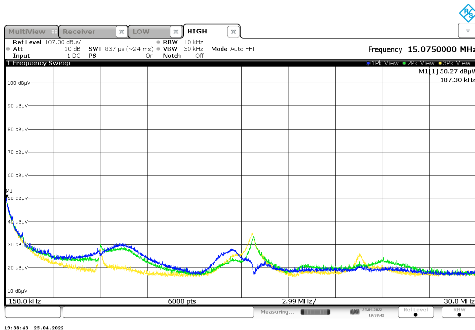
Figure 2.8.6-4: Reference plot for Radiated Spurious Emissions– 150 kHz – 30MHz
