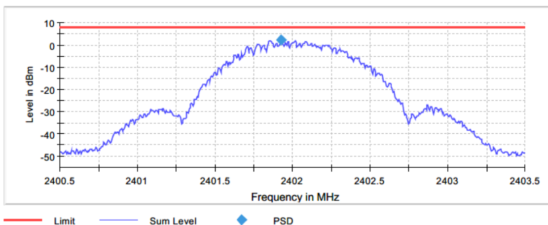
Figure 2.5.6-1: PSD – LCH
