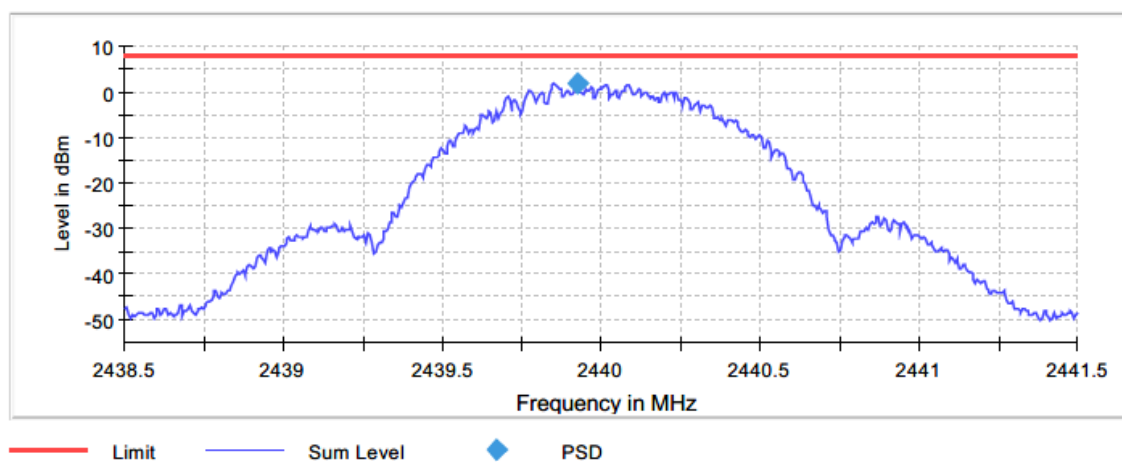
Figure 2.5.6-2: PSD – MCH
