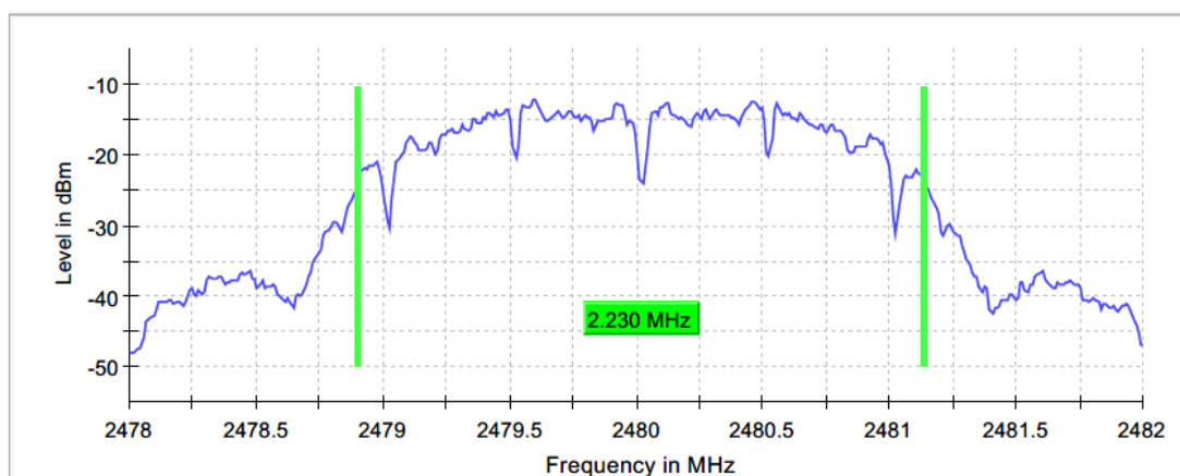
Figure 2.4.6-8: 99% BW - HCH – 2480 MHz
