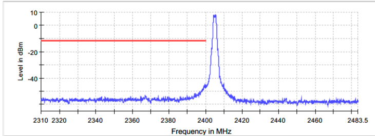
Figure 2.6.6-1: Lower Band-edge – 2405 MHz
