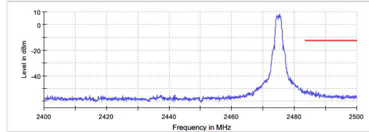
Figure 2.6.6-2: Upper Band-edge – 2475MHz
