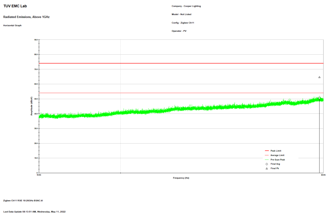
Figure 2.8.6-14: Reference plot for Radiated Spurious Emissions – 18 GHz – 26 GHz – H polarity
