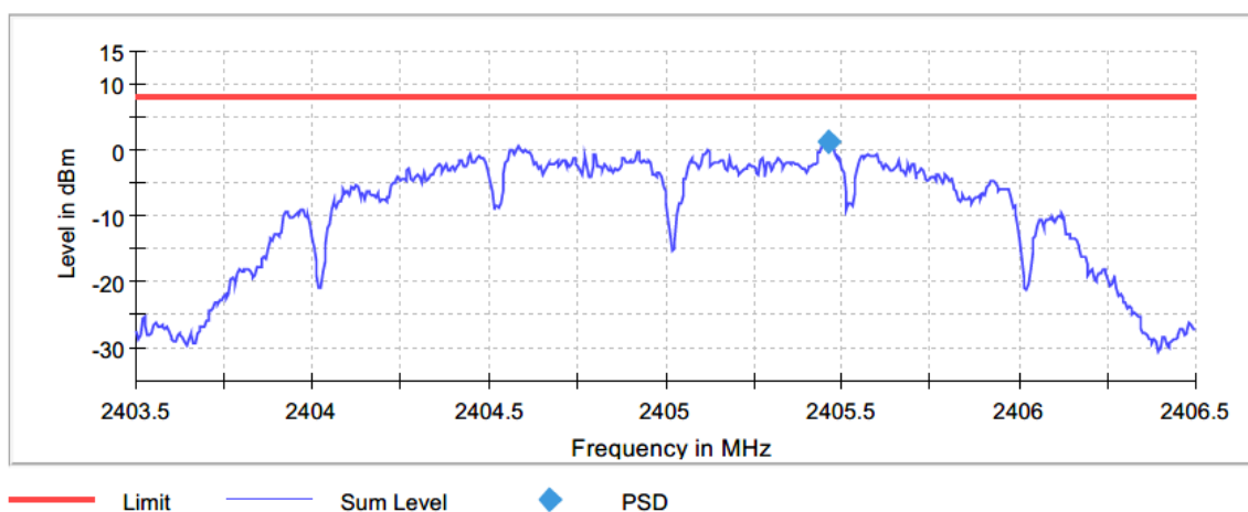
Figure 2.5.6-1: PSD – LCH – 2405 MHz
