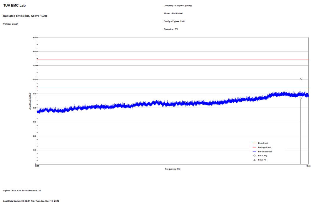
Figure 2.8.6-13: Reference plot for Radiated Spurious Emissions – 10 GHz – 18 GHz – V polarity
