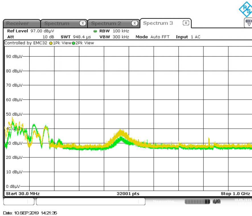
Figure A-3: 30MHz-1GHz
