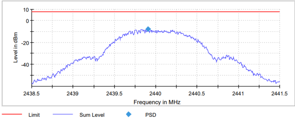
Figure 2.5.6-2: PSD – MCH
