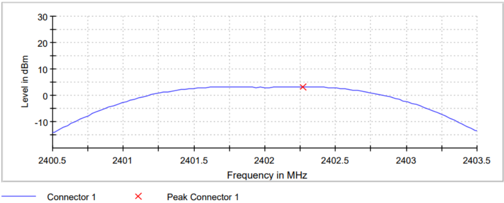
Figure 2.3.6-1: Output Power - LCH
