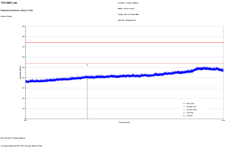
Figure 2.8.6-12: Reference plot for Radiated Spurious Emissions – 10 GHz – 18 GHz – V polarity
