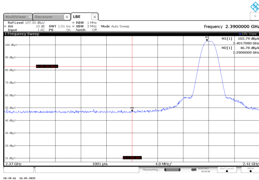
Figure 2.8.6-1: Radiated Lower Band-edge – LCH
