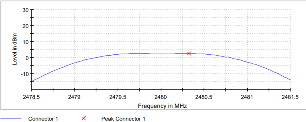
Figure 2.3.6-3: Output Power - HCH
