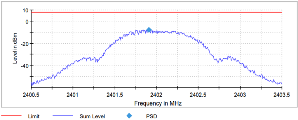
Figure 2.5.6-1: PSD – LCH
