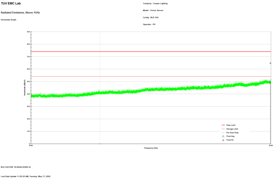
Figure 2.8.6-13: Reference plot for Radiated Spurious Emissions – 18 GHz – 26 GHz – H Polarity
