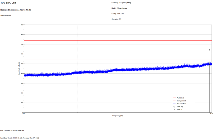
Figure 2.8.6-14: Reference plot for Radiated Spurious Emissions – 18 GHz – 26 GHz – V Polarity
