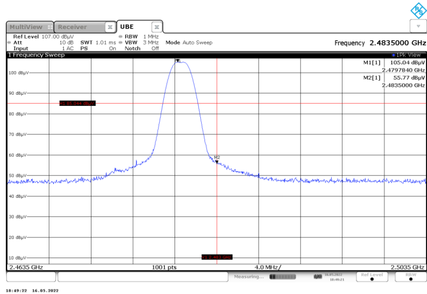
Figure 2.8.6-2: Radiated Upper Band-edge – HCH
