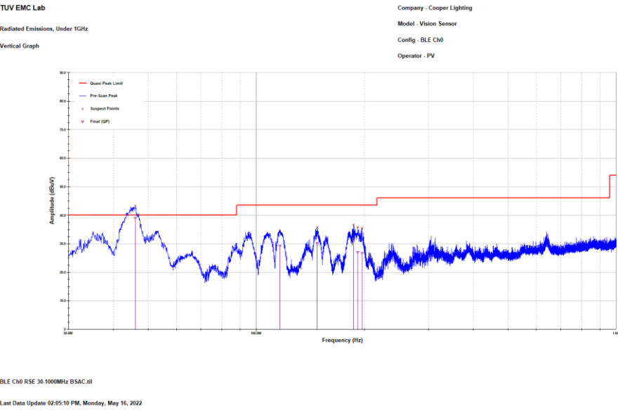
Figure 2.8.6-6: Reference plot for Radiated Spurious Emissions – 30 MHz – 1 GHz – V Polarity Note: Frequencies that falls under restricted band are only evaluated and reported. Emission above the limit line is ambient noise not associated with the radio of the EUT.
