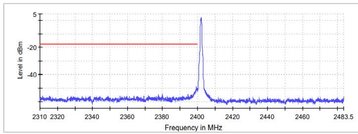
Figure 2.6.6-1: Lower Band-edge
