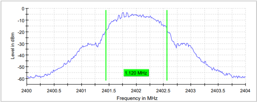
Figure 2.4.6-4: 99% BW - LCH
