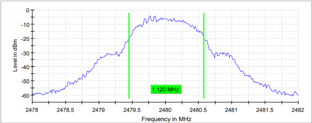
Figure 2.4.6-6: 99% BW - HCH
