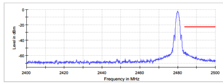
Figure 2.6.6-2: Upper Band-edge
