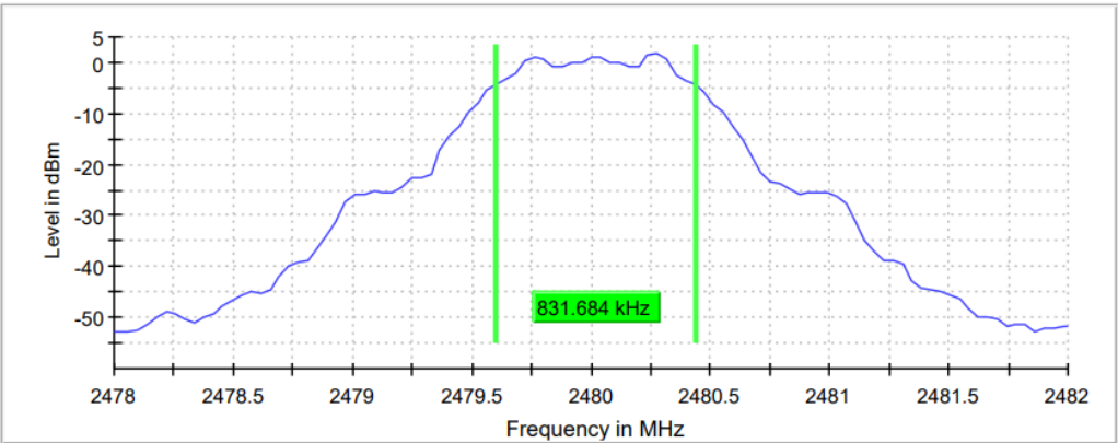
Figure 2.4.6-3: 6 dB BW - HCH
