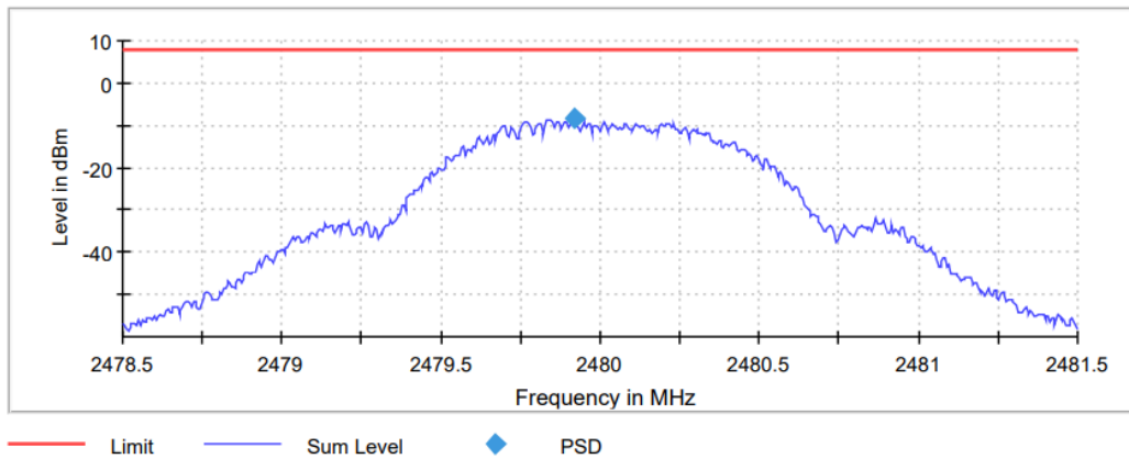
Figure 2.5.6-3: PSD – HCH
