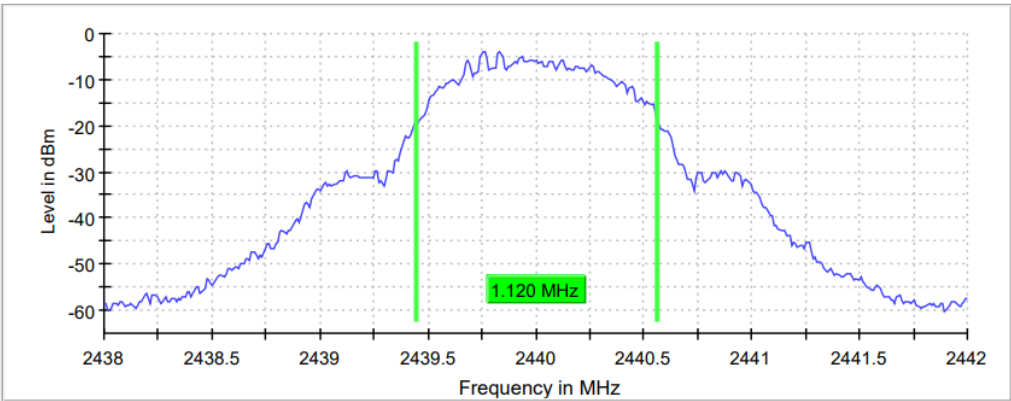
Figure 2.4.6-5: 99% BW - MCH
