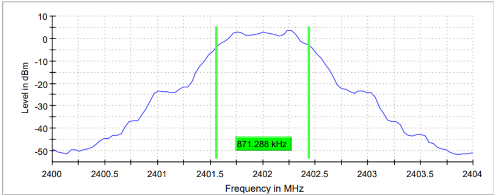
Figure 2.4.6-1: 6 dB BW - LCH
