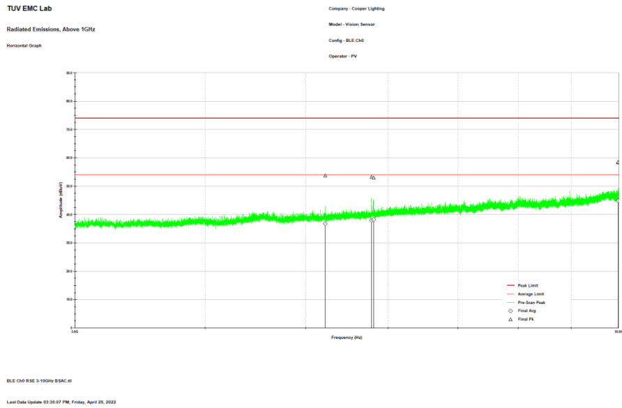
Figure 2.8.6-9: Reference plot for Radiated Spurious Emissions – 3 GHz – 10 GHz – H Polarity
