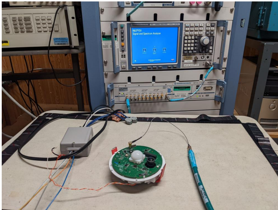
Figure 7: Test Setup – Antenna Port Measurements
