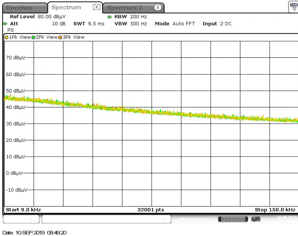
Figure A-1: 9kHz-150kHz
