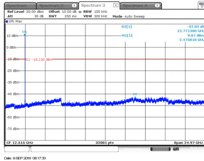
Figure 7.5.1.2-3: HCH – 30MHz–25GHz
