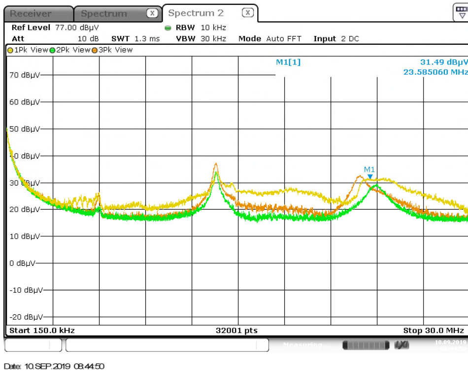
Figure A-2: 150kHz-30MHz
