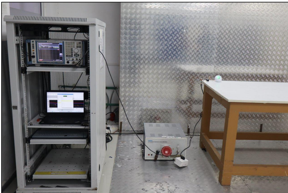
Conducted AC Powerline Test Setup
