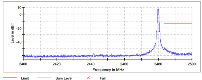
Figure 2.6.6-2: Upper Band-edge - 1 Mbps
