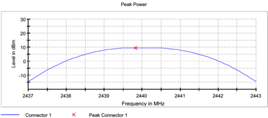
Figure 2.3.6-2: Output Power - MCH
