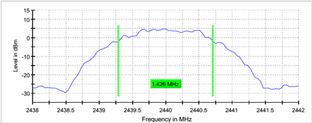
Figure 2.4.6-8: 6 dB BW - MCH
