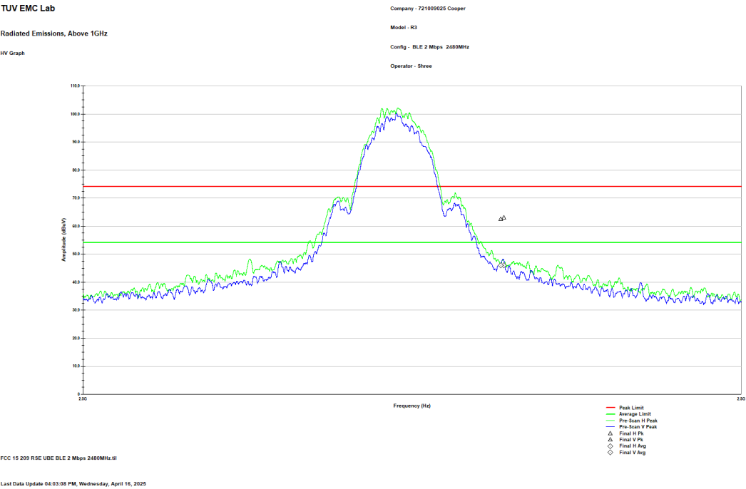
Figure 2.8.6-4: Radiated Upper Band-edge – HCH – 2Mbps
