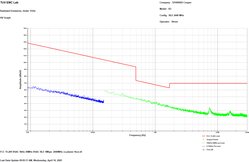
Figure 2.8.6-6: Reference plot for Radiated Spurious Emissions – 9 kHz – 30 MHz – 1Mbps – Co-Planar Horizontal
