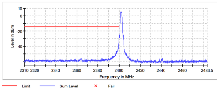
Figure 2.6.6-3: Lower Band-edge – 2 Mbps
