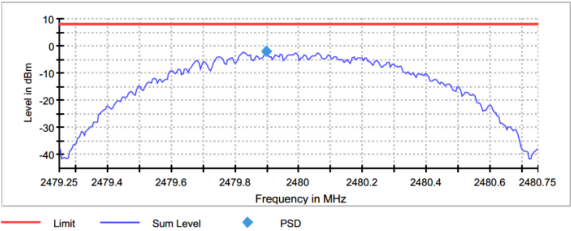
Figure 2.5.6-3: PSD – HCH
