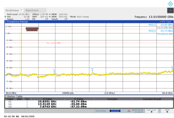
Figure 2.7.6-4: 30MHz – 26GHz – LCH – 2Mbps
