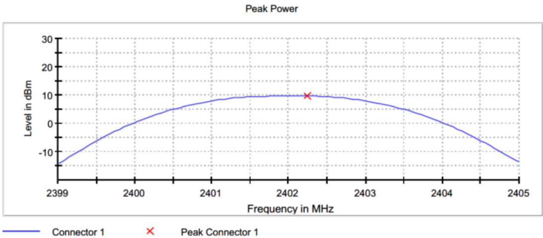
Figure 2.3.6-1: Output Power - LCH
