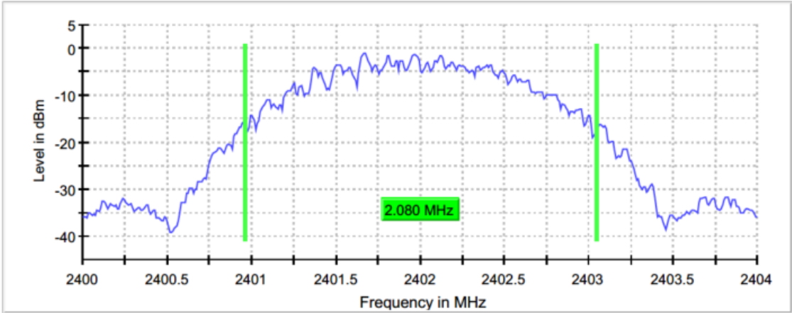
Figure 2.4.6-10: 99% BW - LCH
