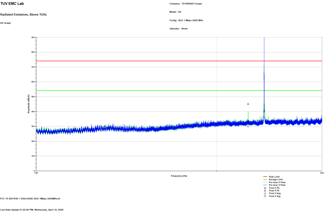
Figure 2.8.6-9: Reference plot for Radiated Spurious Emissions – 1 GHz – 3 GHz – 1Mbps Note: Emission above the limit line is the Fundamental Frequency.
