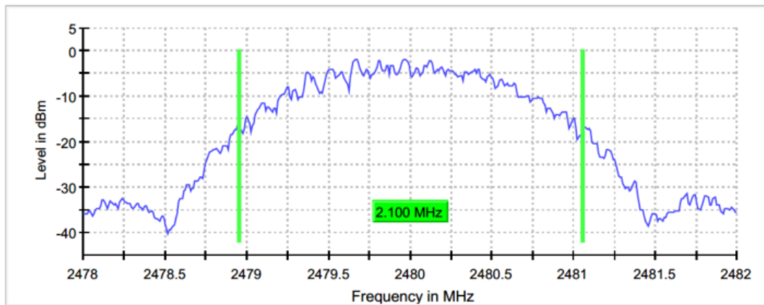
Figure 2.4.6-12: 99% BW - HCH
