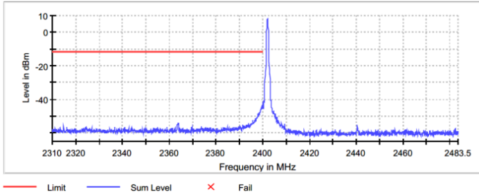
Figure 2.6.6-1: Lower Band-edge – 1 Mbps
