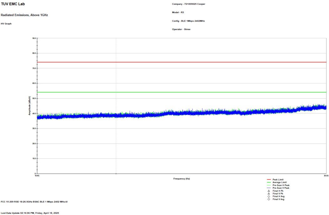
Figure 2.8.6-12: Reference plot for Radiated Spurious Emissions – 18 GHz – 26.5 GHz – 1Mbps
