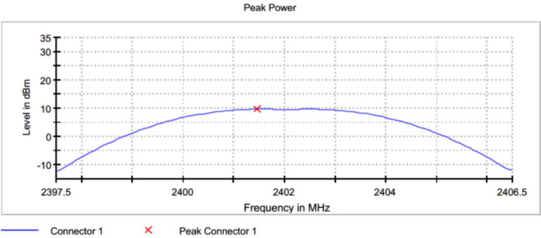
Figure 2.3.6-4: Output Power - LCH
