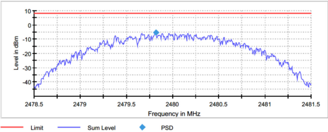
Figure 2.5.6-6: PSD – HCH
