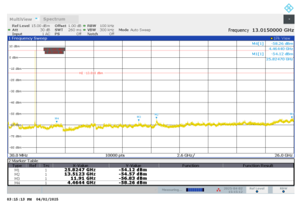
Figure 2.7.6-6: 30MHz – 26GHz – HCH – 2Mbps
