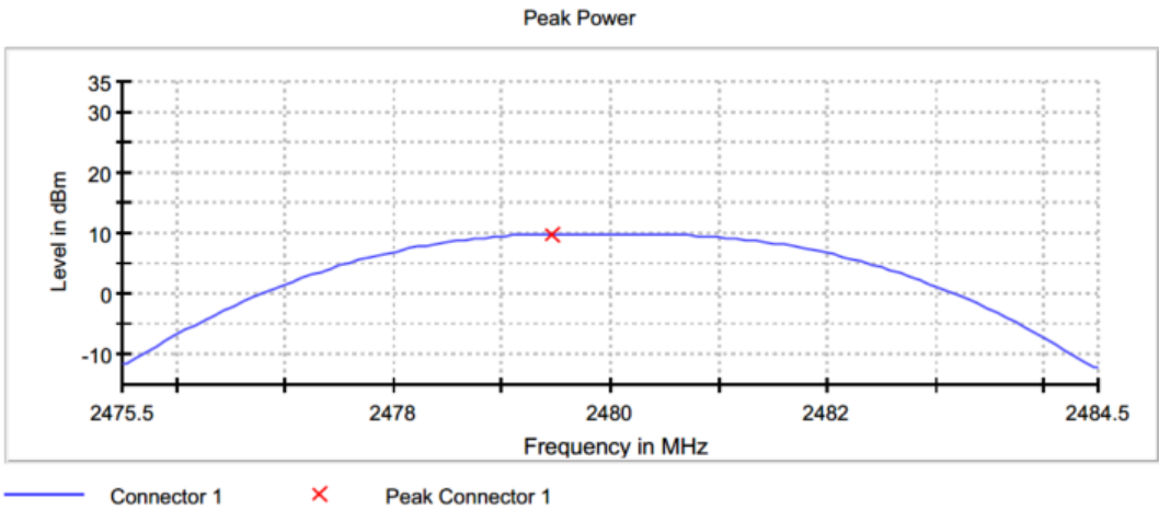
Figure 2.3.6-6: Output Power - HCH
