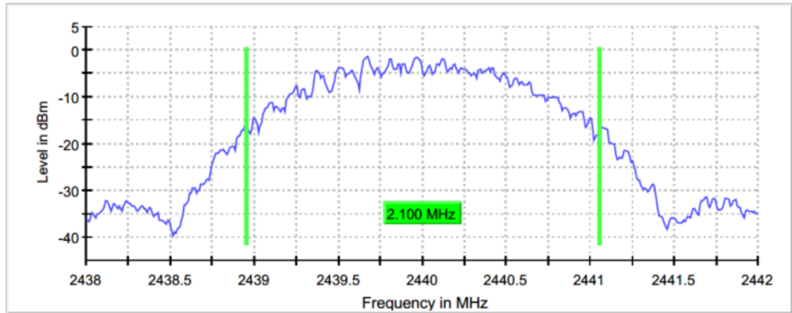
Figure 2.4.6-11: 99% BW - MCH
