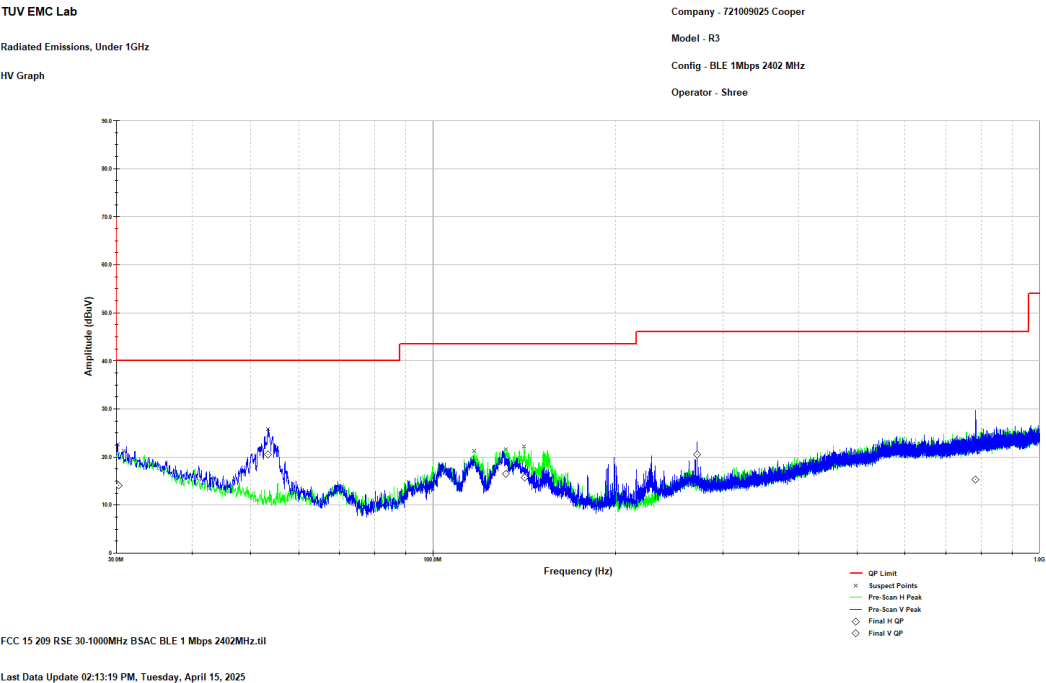
Figure 2.8.6-8: Reference plot for Radiated Spurious Emissions – 30 MHz – 1 GHz – 1Mbps Note: Frequencies that fall under restricted band are only evaluated and reported.
