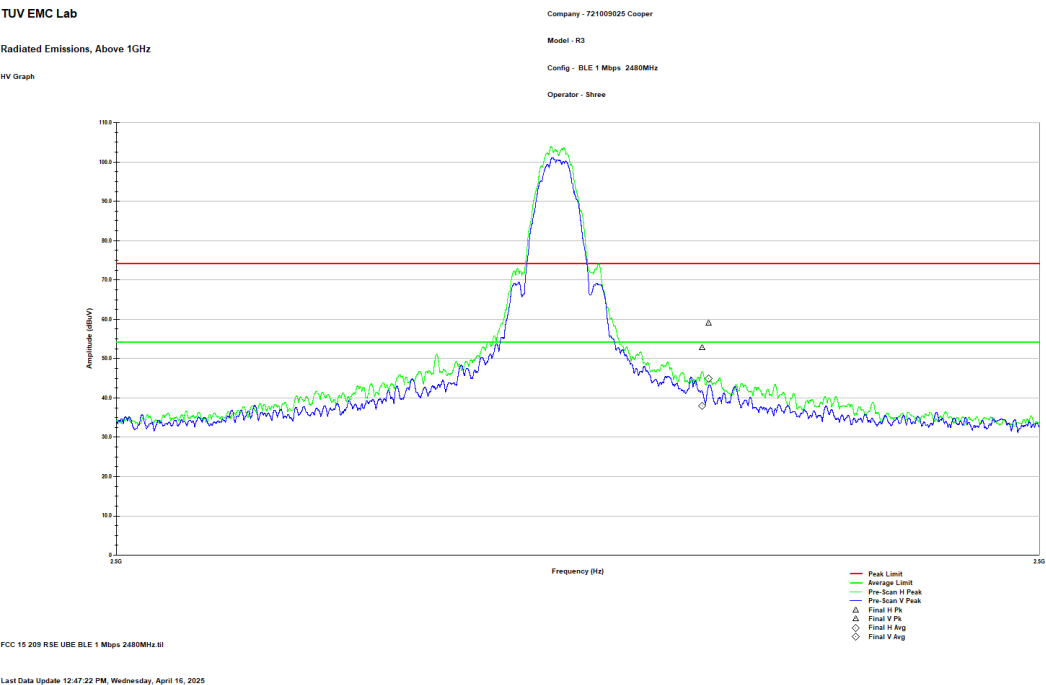
Figure 2.8.6-2: Radiated Upper Band-edge – HCH – 1Mbps
