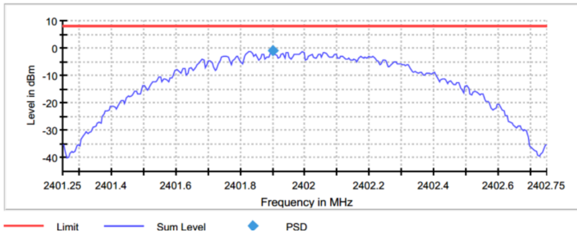
Figure 2.5.6-1: PSD – LCH
