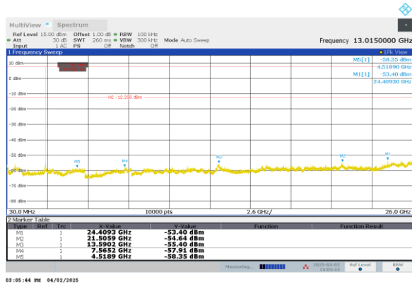
Figure 2.7.6-3: 30MHz – 26GHz – HCH – 1Mbps
