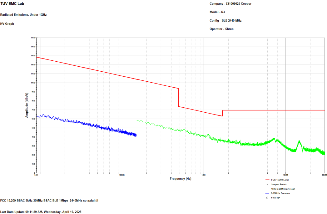
Figure 2.8.6-5: Reference plot for Radiated Spurious Emissions – 9 kHz – 30 MHz – 1Mbps – Co-axial
