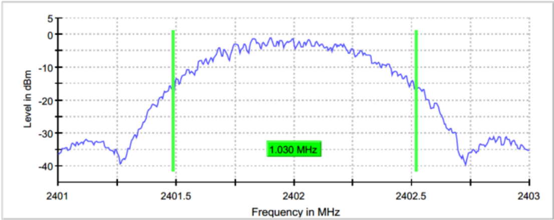
Figure 2.4.6-4: 99% BW - LCH
