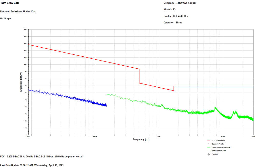
Figure 2.8.6-7: Reference plot for Radiated Spurious Emissions – 9 kHz – 30 MHz – 1Mbps – Co-Planar Vertical
