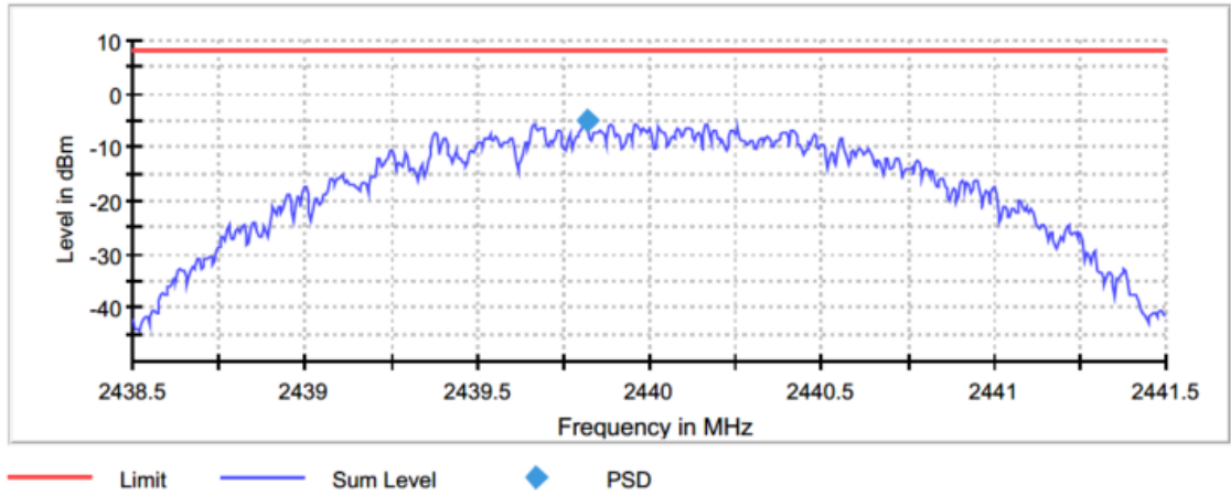
Figure 2.5.6-5: PSD – MCH
