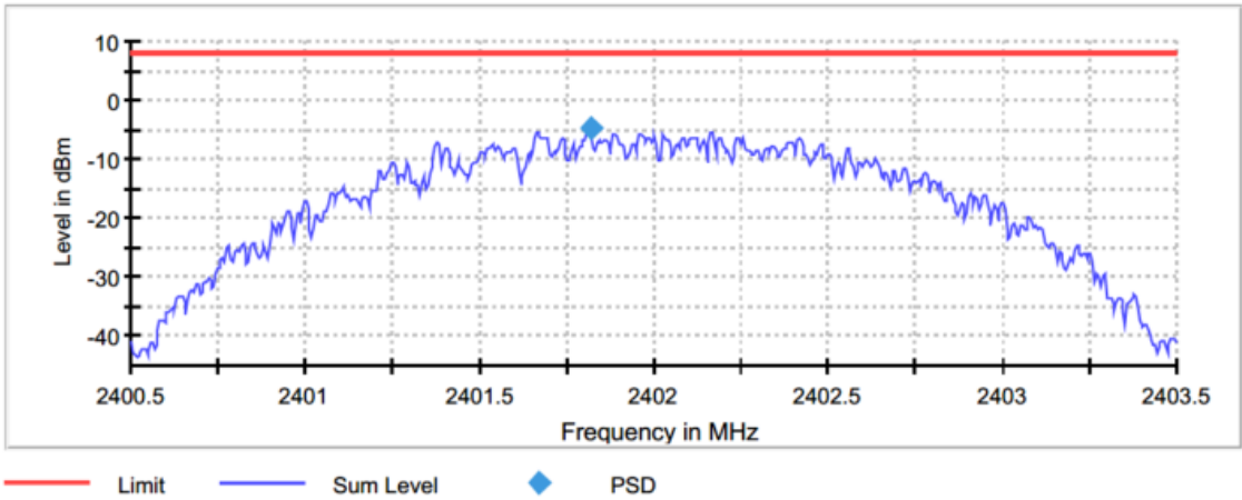
Figure 2.5.6-4: PSD – LCH
