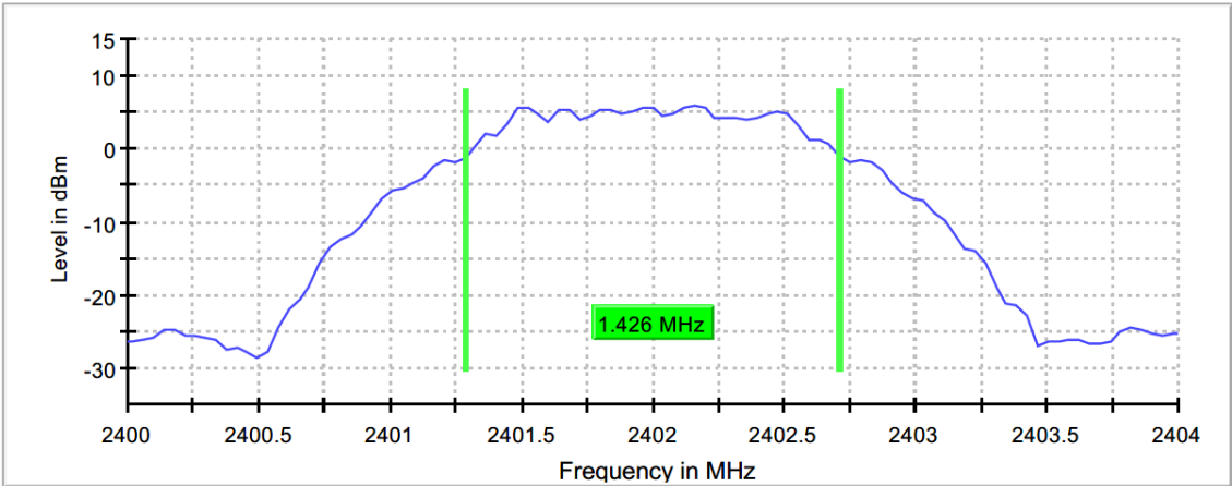
Figure 2.4.6-7: 6 dB BW - LCH
