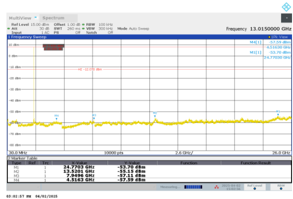
Figure 2.7.6-2: 30MHz – 26GHz – MCH – 1Mbps
