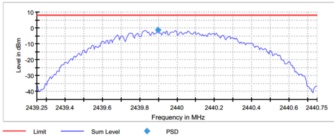
Figure 2.5.6-2: PSD – MCH
