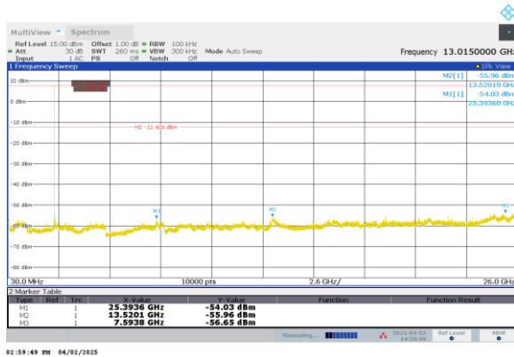
Figure 2.7.6-1: 30MHz – 26GHz – LCH – 1Mbps
