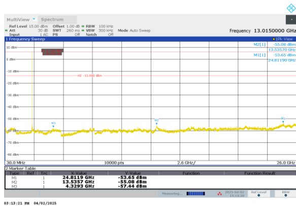
Figure 2.7.6-5: 30MHz – 26GHz – MCH – 2Mbps
