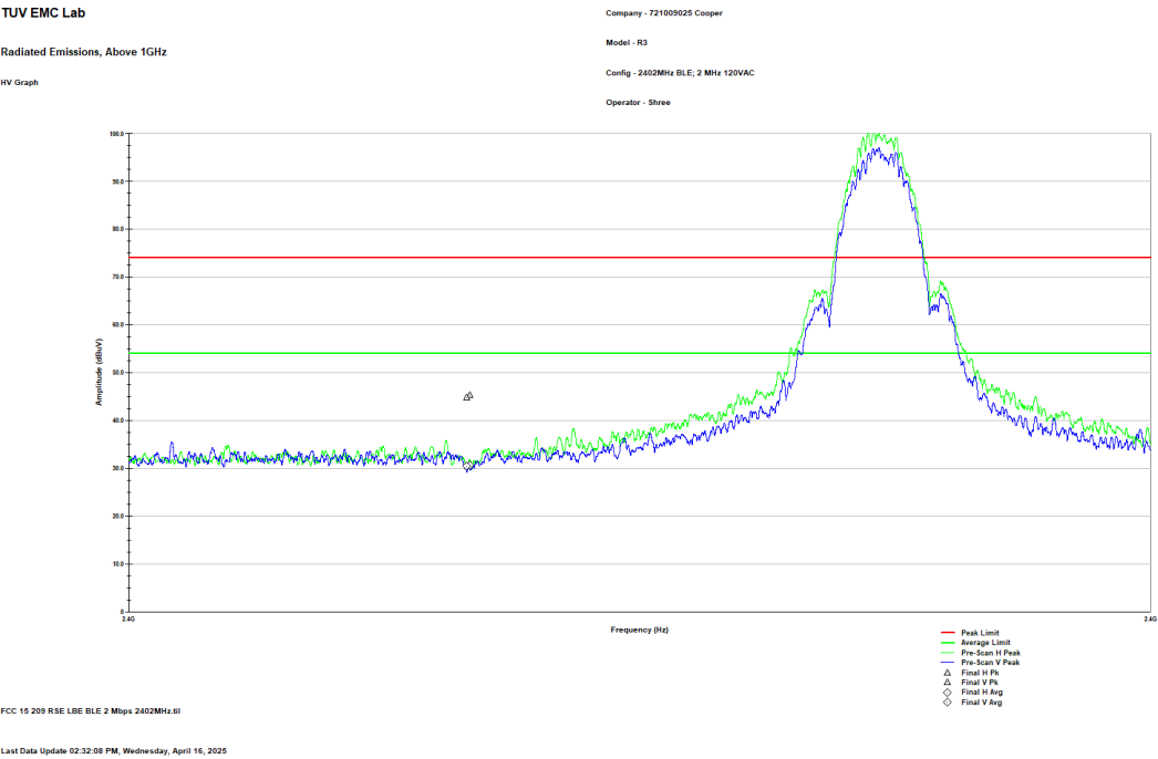
Figure 2.8.6-3: Radiated Lower Band-edge – LCH – 2Mbps
