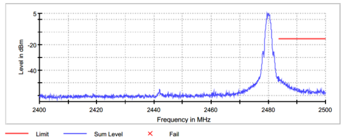
Figure 2.6.6-4: Upper Band-edge - 2 Mbps
