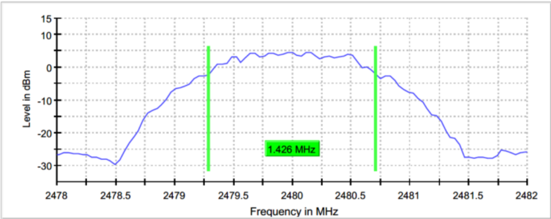
Figure 2.4.6-9: 6 dB BW - HCH
