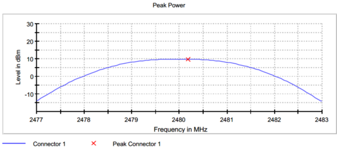
Figure 2.3.6-3: Output Power - HCH
