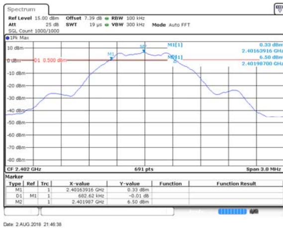
GFSK (BLE) LOW CHANNEL
