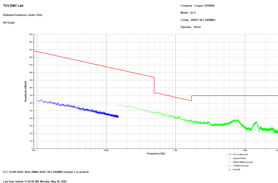
Figure 2.8.6-10: Reference plot for Radiated Spurious Emissions – 9 kHz – 30 MHz
