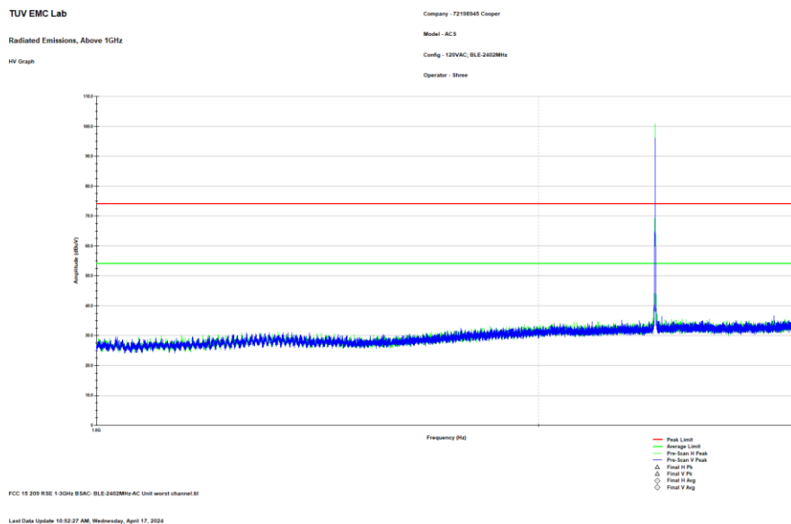
Figure 2.8.6-12: Reference plot for Radiated Spurious Emissions – 1 GHz – 3 GHz
