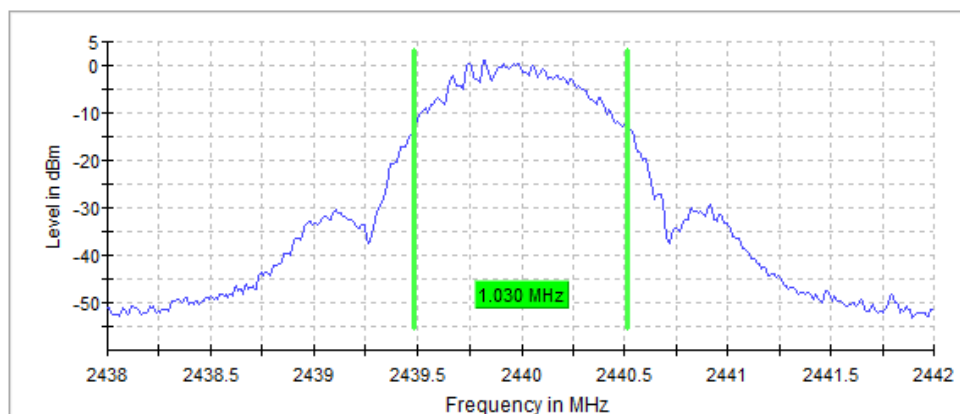
Figure 2.4.6-5: 99% BW - MCH
