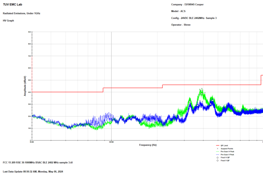
Figure 2.8.6-4: Reference plot for Radiated Spurious Emissions – 30 MHz – 1 GHz
