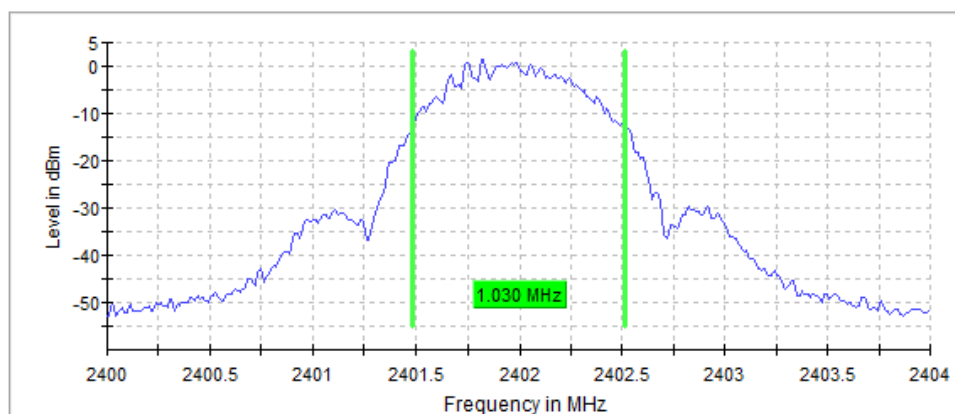
Figure 2.4.6-4: 99% BW - LCH
