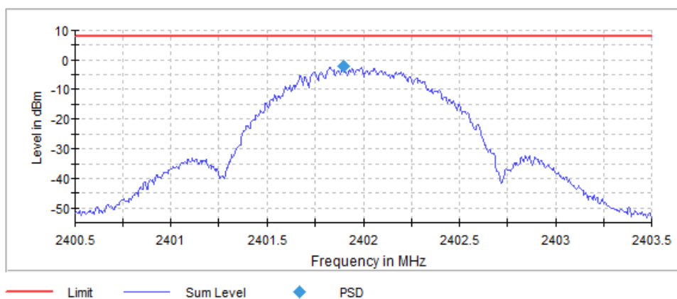
Figure 2.5.6-1: PSD – LCH
