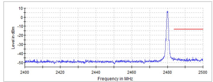
Figure 2.6.6-2: Upper Band-edge
