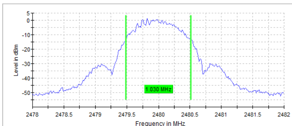
Figure 2.4.6-6: 99% BW - HCH
