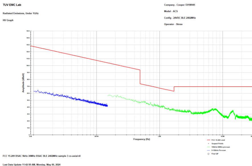
Figure 2.8.6-3: Reference plot for Radiated Spurious Emissions – 9 kHz – 30 MHz
