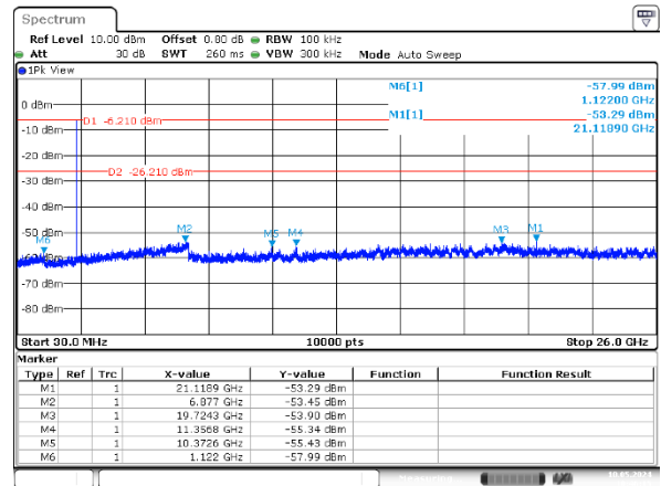
Figure 2.7.6-2: 30MHz – 26GHz – MCH
