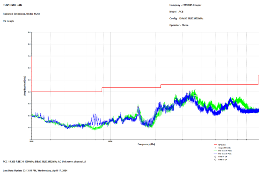
Figure 2.8.6-11: Reference plot for Radiated Spurious Emissions – 30 MHz – 1 GHz
