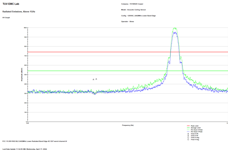
Figure 2.8.6-9: Radiated Lower Band-edge – LCH
