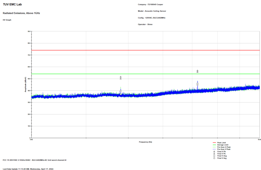
Figure 2.8.6-13: Reference plot for Radiated Spurious Emissions – 3 GHz – 10 GHz
