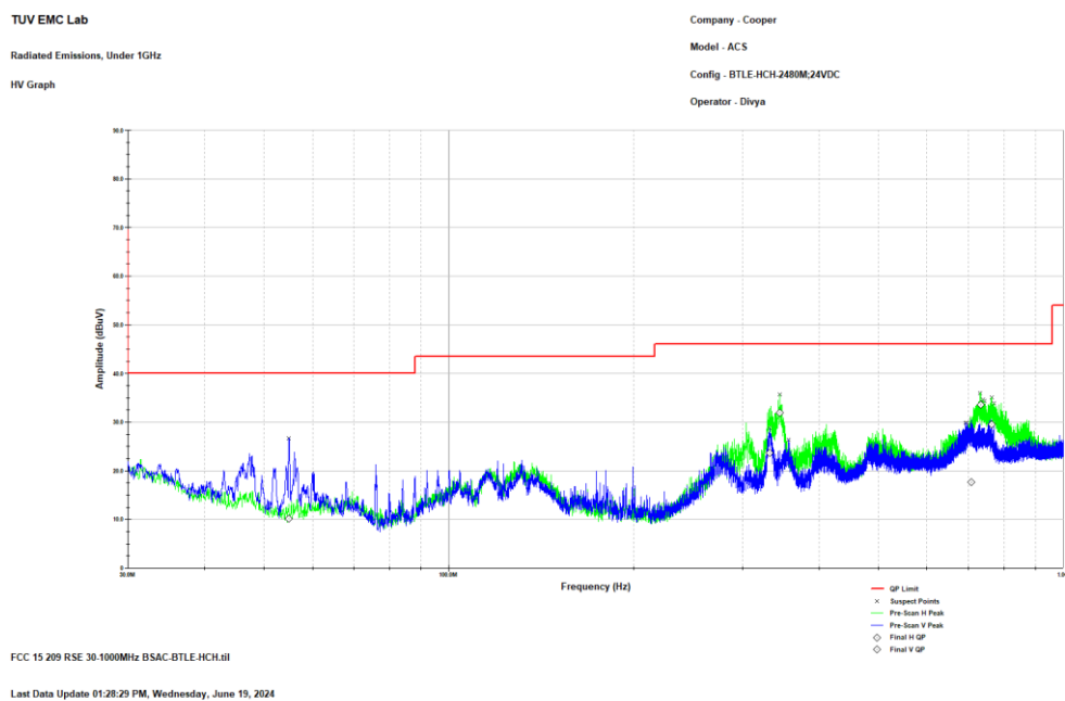
Figure 2.3.6-3: Radiated Spurious Emissions – 30 MHz – 1 GHz - HCH
