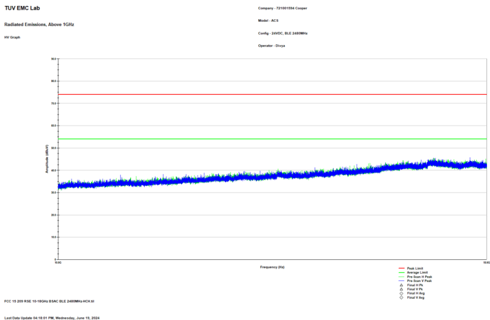
Figure 2.3.6-6: Radiated Spurious Emissions – 10 GHz – 18 GHz - HCH
