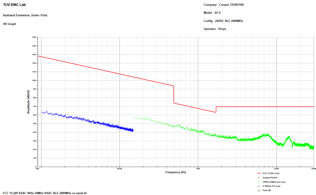
Figure 2.3.6-2: Radiated Spurious Emissions – 9 kHz – 30 MHz - HCH
