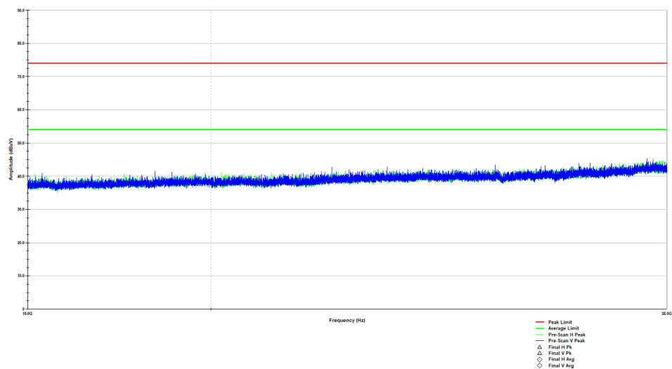
Figure 2.3.6-7: Radiated Spurious Emissions – 18 GHz – 26 GHz - HCH
