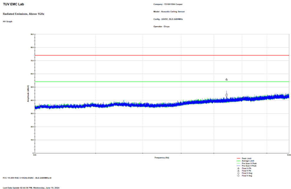
Figure 2.3.6-5: Radiated Spurious Emissions – 3 GHz – 10 GHz - HCH
