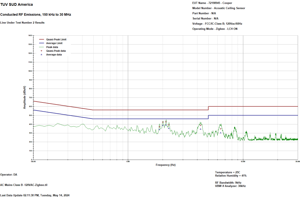
Figure 2.2.6-2: Conducted Emission Plot – Nuetral
