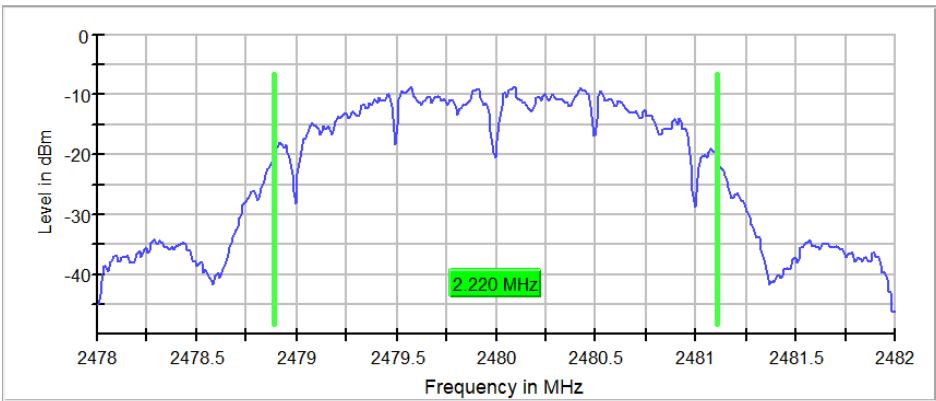
Figure 2.4.6-8: 99% BW - HCH – 2480 MHz
