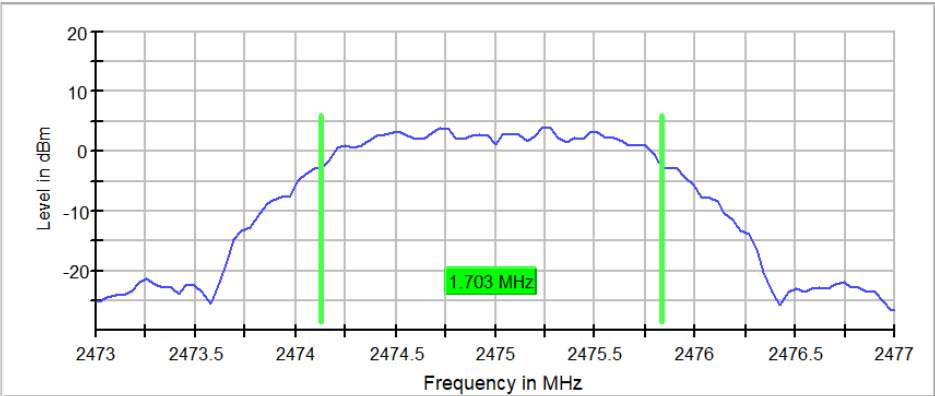
Figure 2.4.6-3: 6 dB BW - HCH – 2475 MHz
