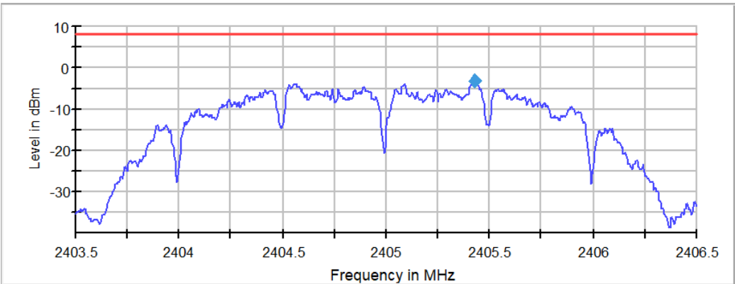
Figure 2.5.6-1: PSD – LCH
