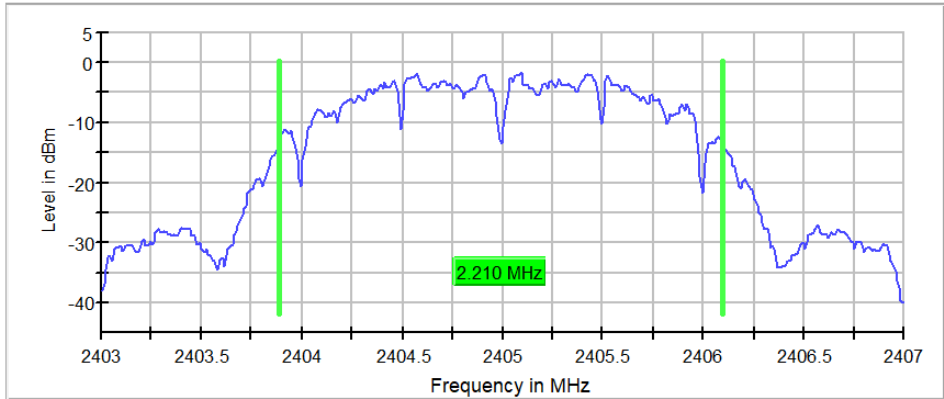
Figure 2.4.6-5: 99% BW - LCH
