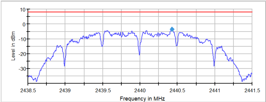
Figure 2.5.6-2: PSD – MCH
