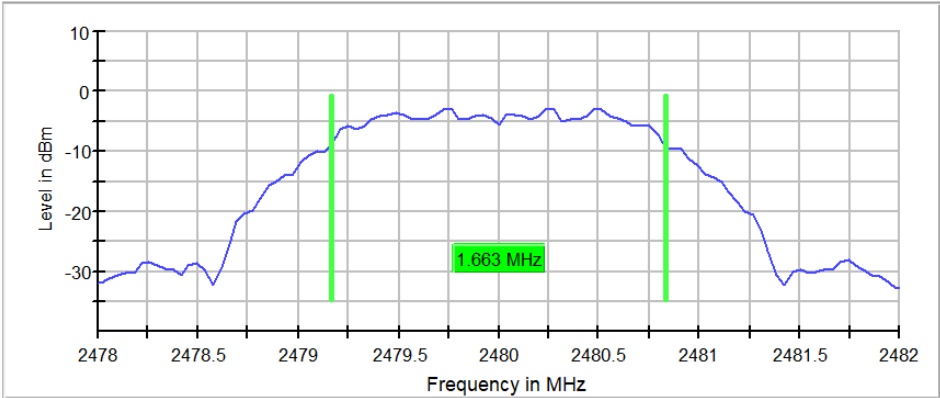
Figure 2.4.6-4: 6 dB BW - HCH – 2480 MHz
