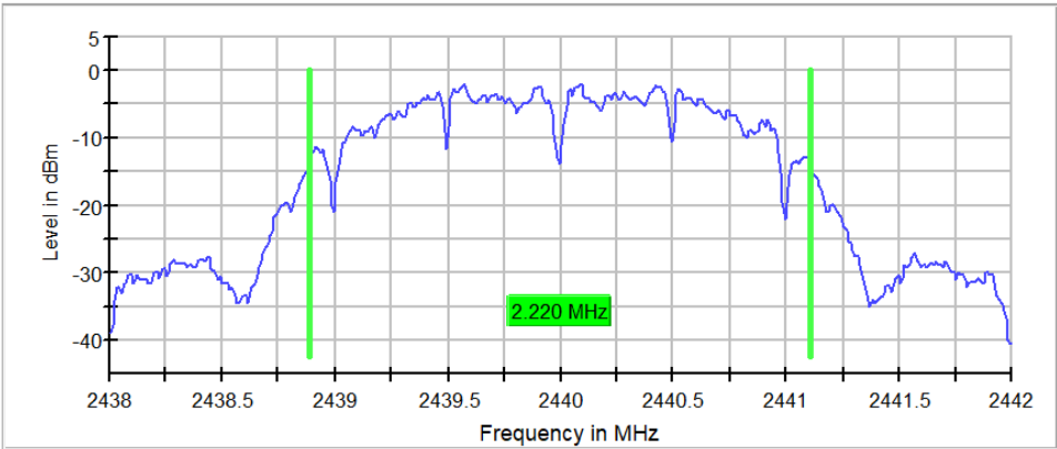
Figure 2.4.6-6: 99% BW - MCH
