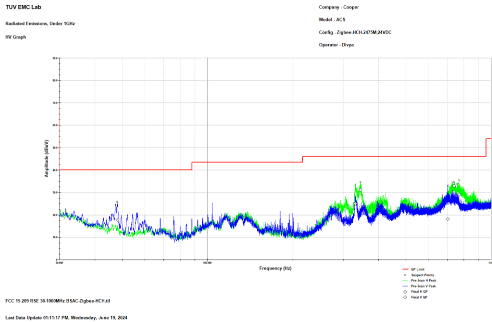
Figure 2.3.6-3: Radiated Spurious Emissions – 30 MHz – 1 GHz - HCH- 2475 MHz
