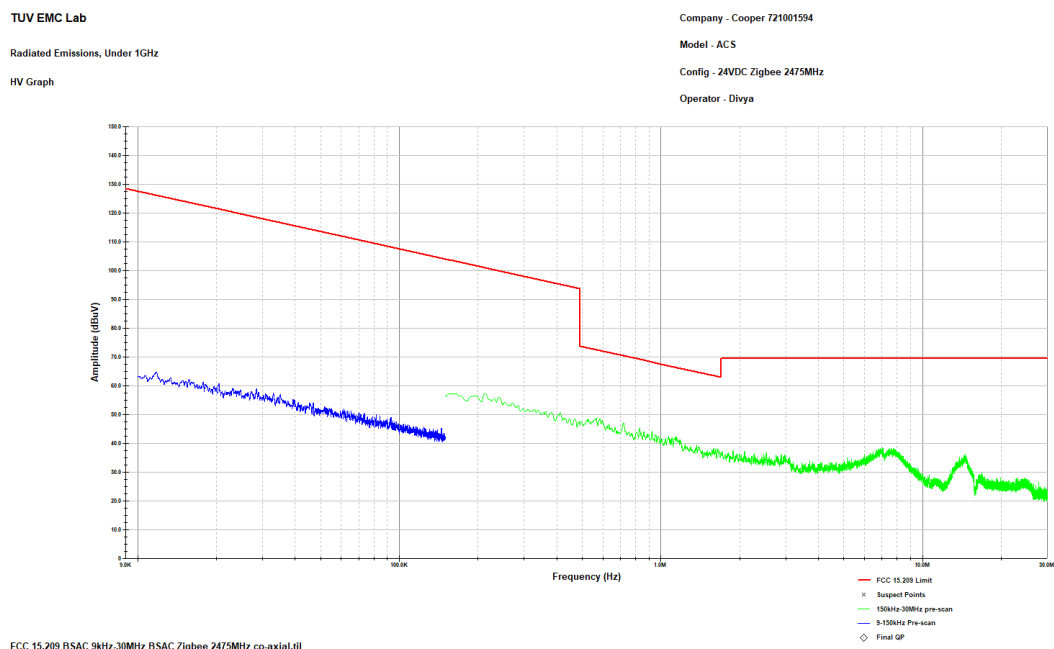
Figure 2.3.6-2: Radiated Spurious Emissions – 9 kHz – 30 MHz - HCH- 2475 MHz
