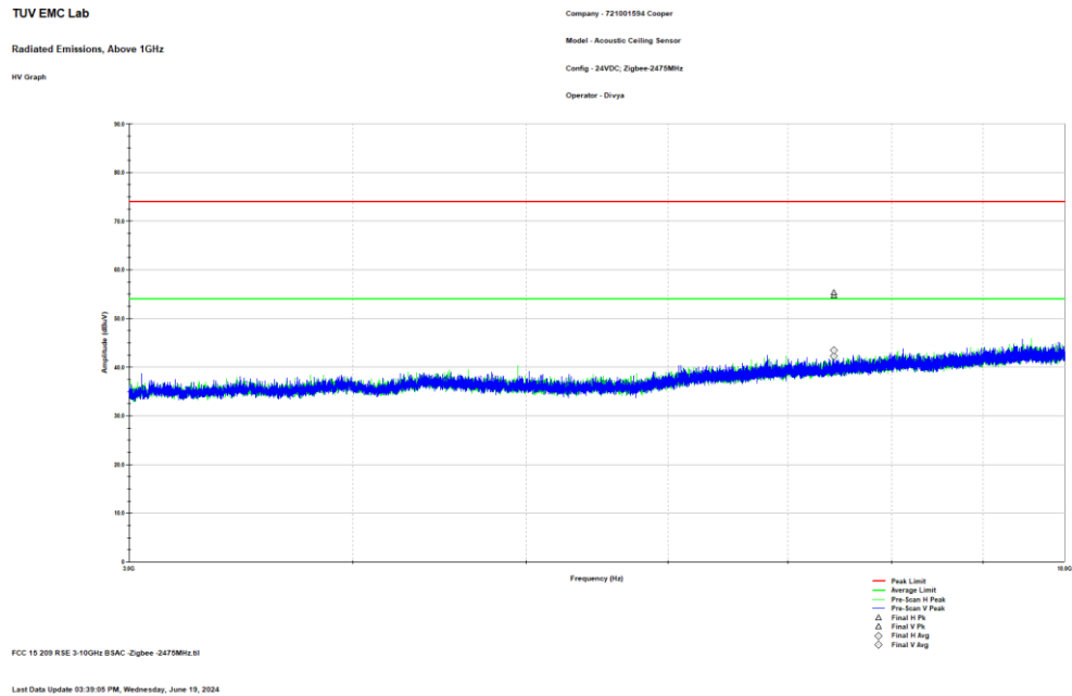
Figure 2.3.6-5: Radiated Spurious Emissions – 3 GHz – 10 GHz - HCH- 2475 MHz
