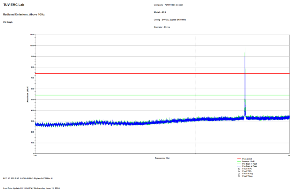
Figure 2.3.6-4: Radiated Spurious Emissions – 1 GHz – 3 GHz - HCH- 2475 MHz Note: Emission above the limit line is the Fundamental Frequency.
