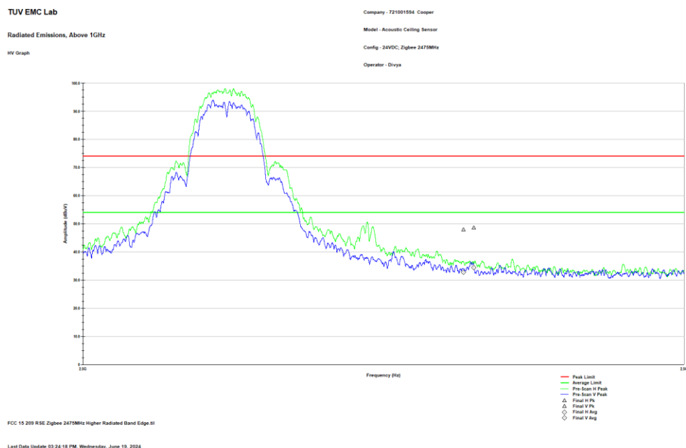
Figure 2.3.6-1: Radiated Upper Band-edge – HCH - 2475 MHz
