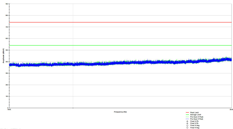
Figure 2.3.6-7: Radiated Spurious Emissions – 18 GHz – 26 GHz - HCH- 2475 MHz
