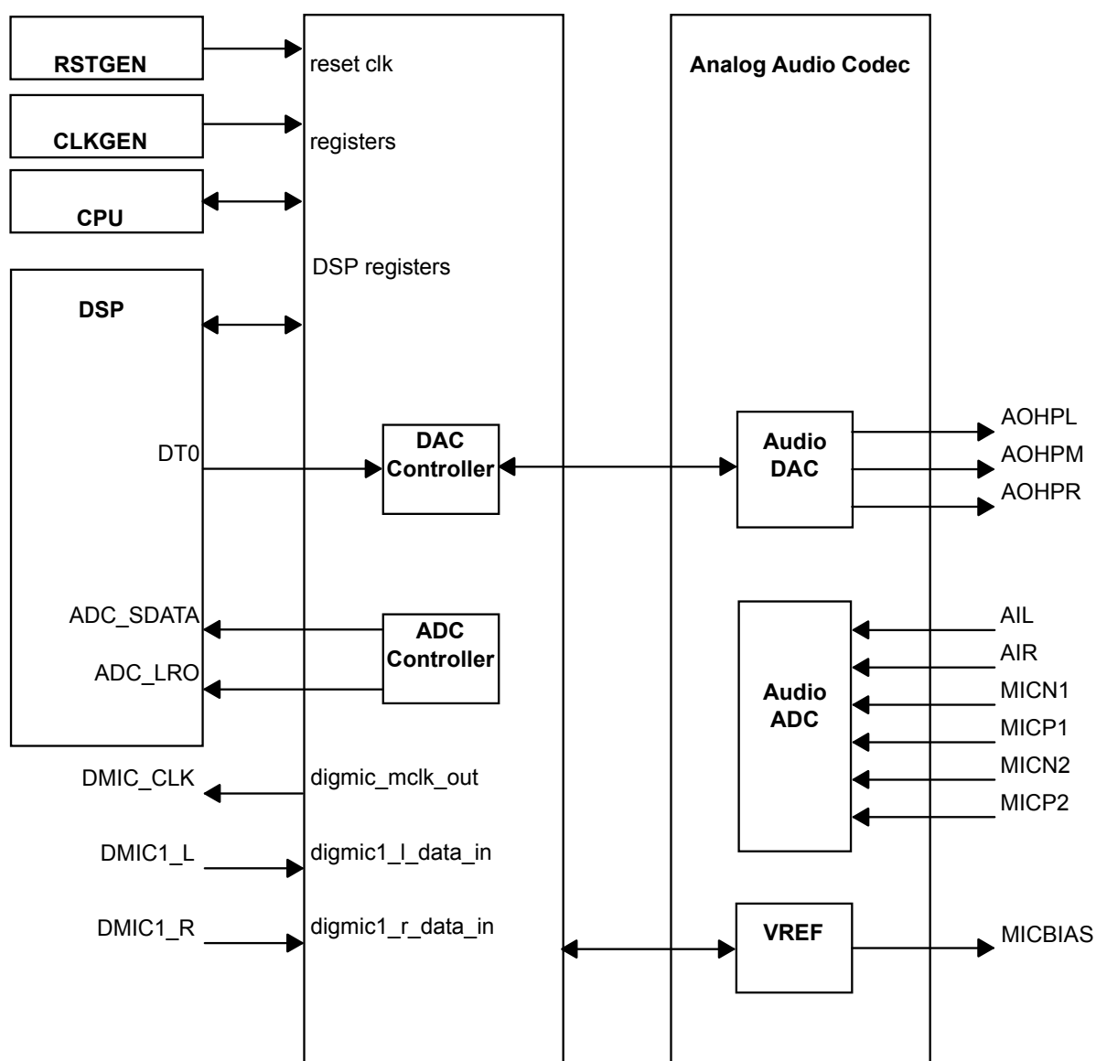
Figure 3-1. Audio Subsystem
