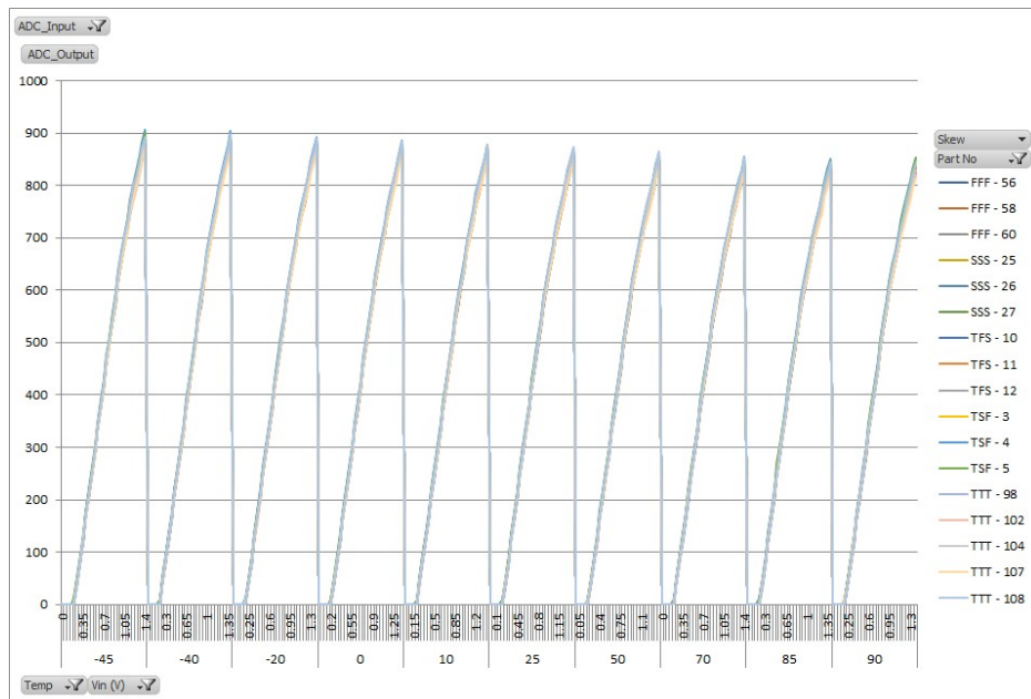
Figure 5-5. SK2 Channel
