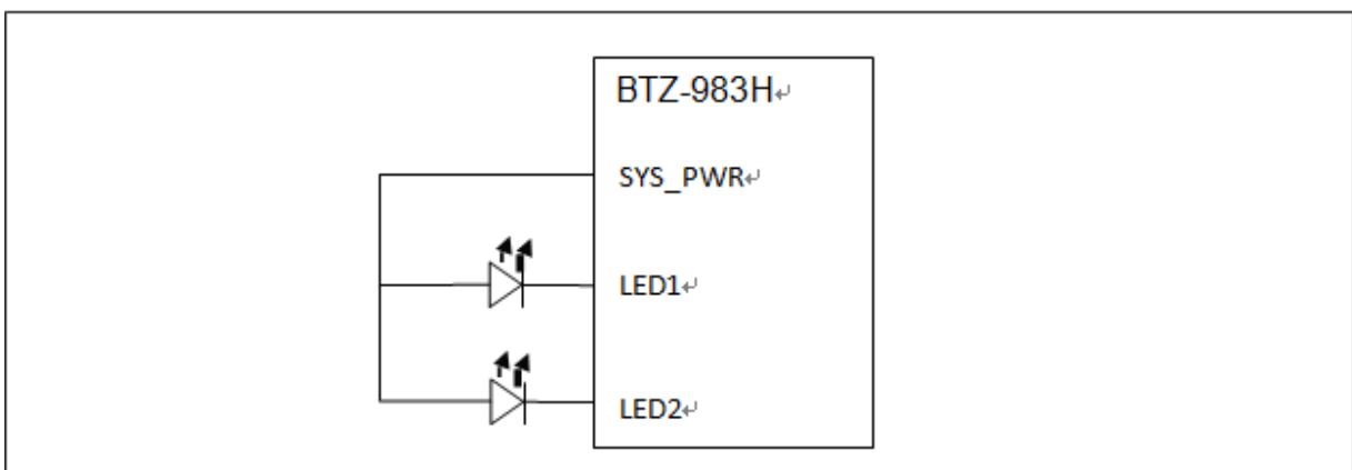
Figure 5-6. LED Drivers
