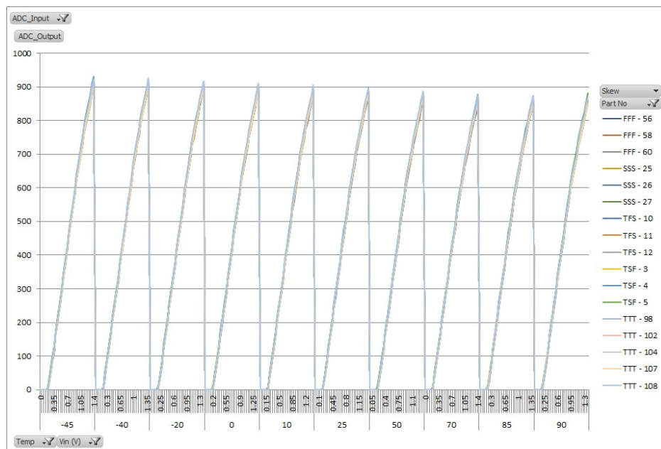
Figure 5-4. SK1 Channel
