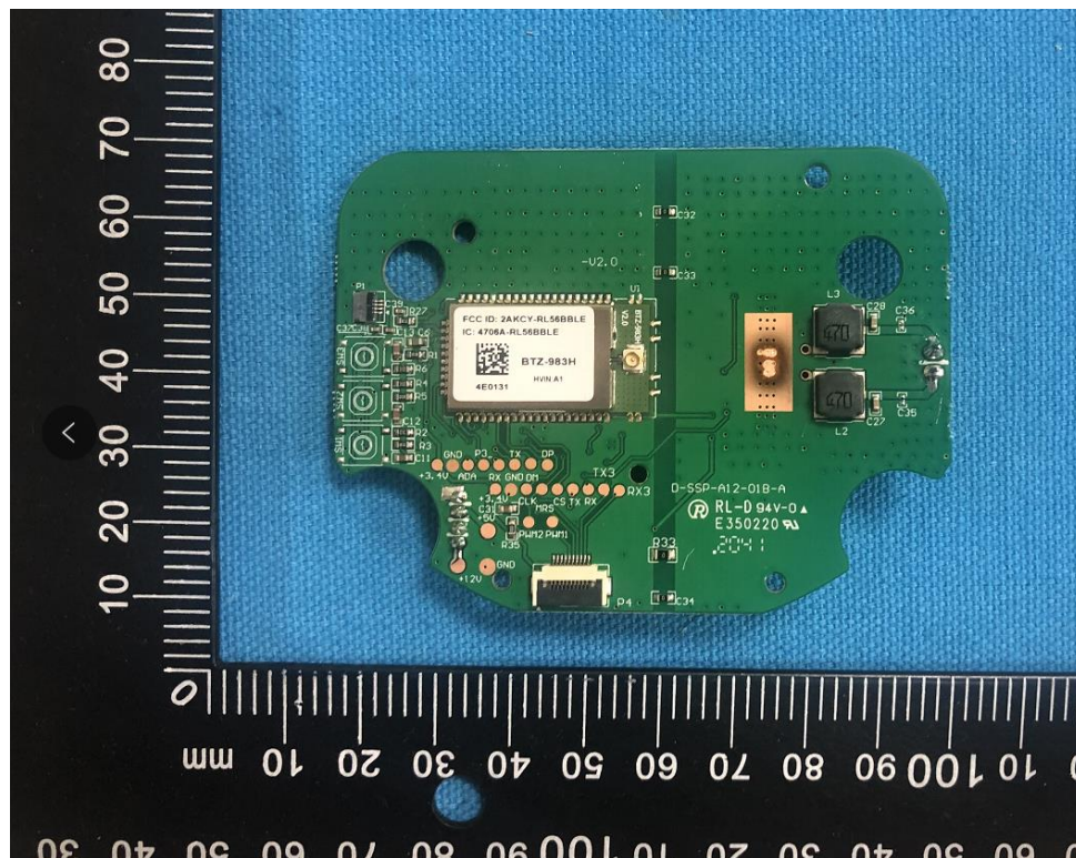
Internal View of EUT-5
