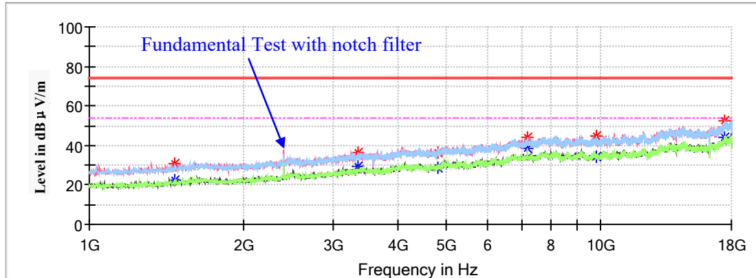
Full Spectrum
