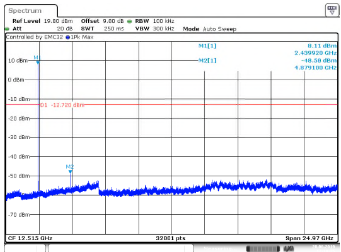
Figure 7.5.1.2-2: MCH – 30MHz–25GHz
