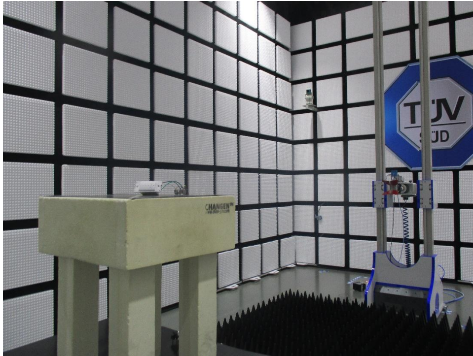
Radiated Emission test of 1-18GHz
