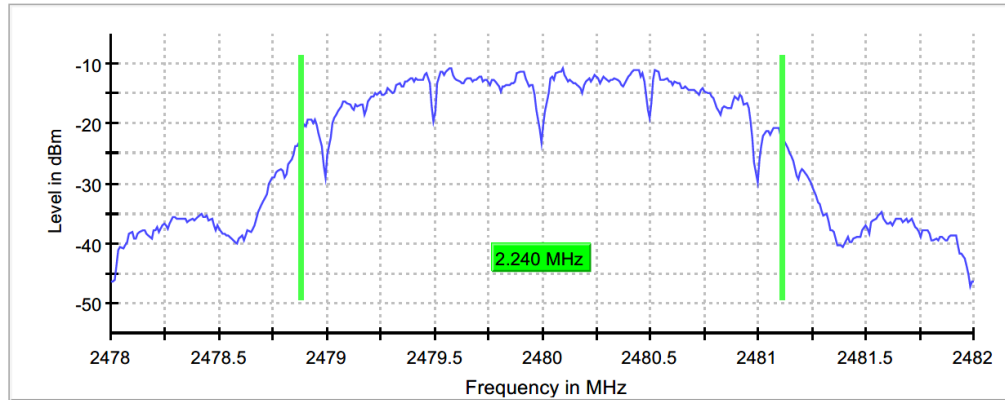
Figure 7.3.2-8: 2480MHz - 99% OBW
