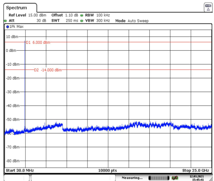
Figure 7.5.1.2-2: MCH (2440MHz) – 30MHz–25GHz
