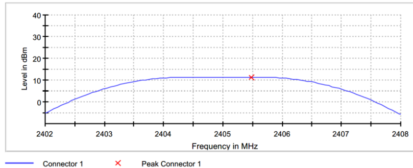
Figure 7.4.2-1: 2405MHz Plot
