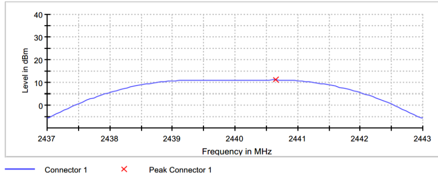
Figure 7.4.2-2: 2440MHz Plot
