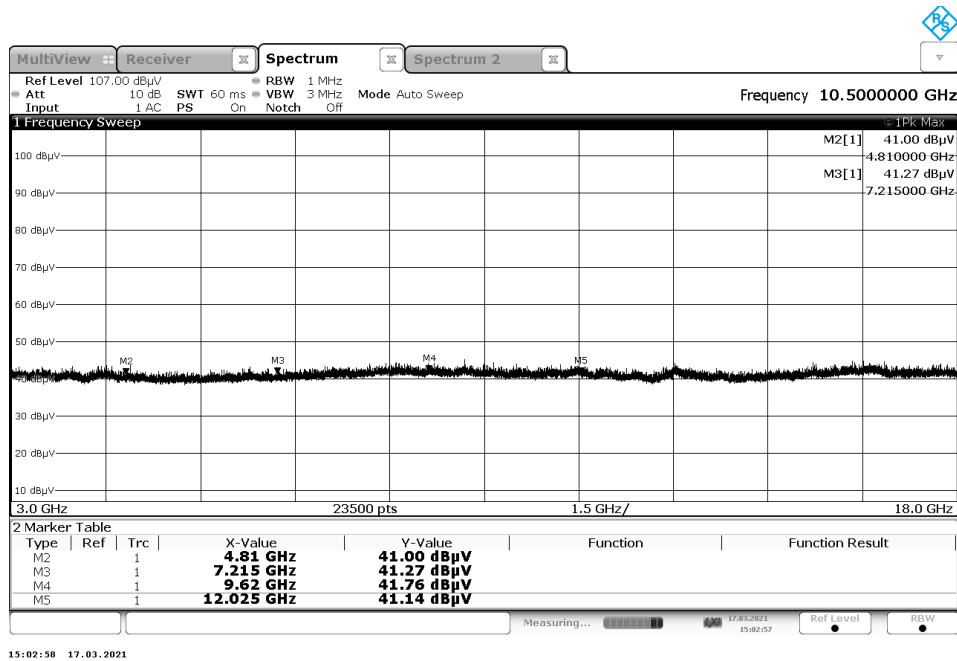
Figure A-5: 3GHz-18GHz
