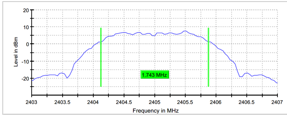
Figure 7.3.2-1: 2405MHz - 6dB BW
