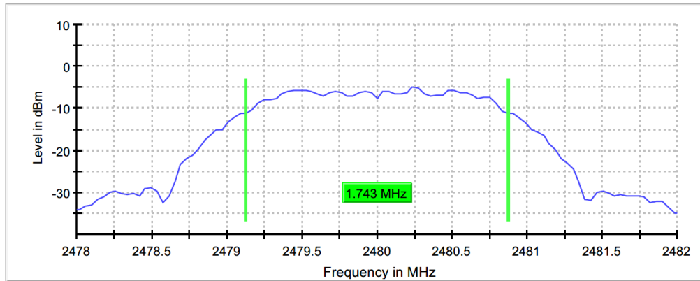
Figure 7.3.2-4: 2480MHz - 6dB BW
