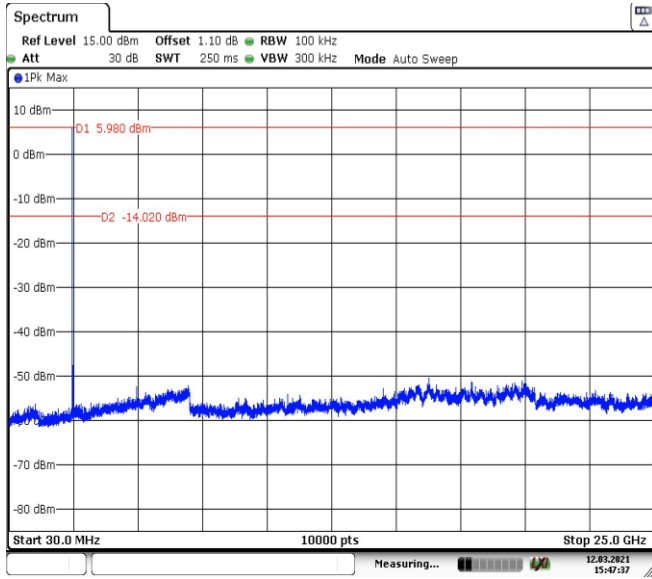
Figure 7.5.1.2-3: HCH (2475MHz) – 30MHz–25GHz
