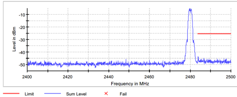
Figure 7.5.1.2-7: Upper Band-edge (2480MHz)
