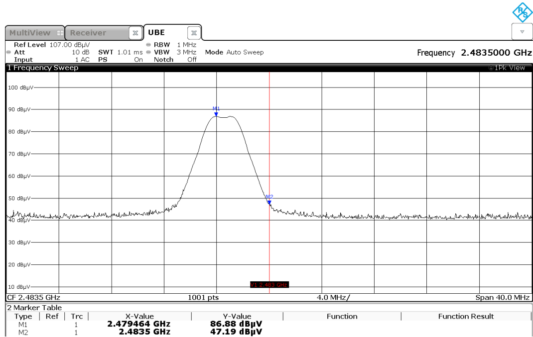
Figure A-9: Restricted Band Edge High – 2480MHz
