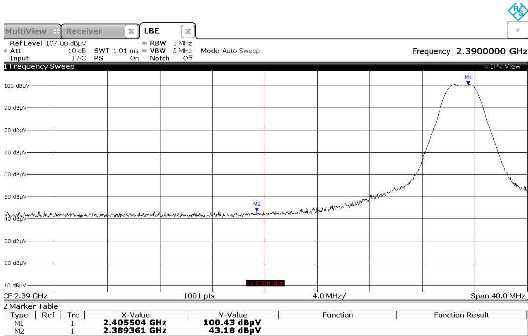
Figure A-7: Restricted Band Edge Low – 2405MHz
