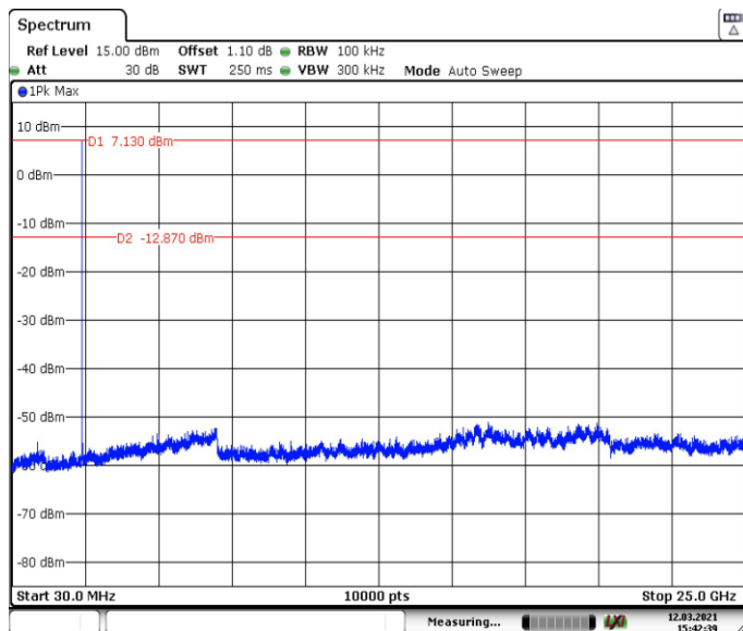
Figure 7.5.1.2-1: LCH (2405MHz) – 30MHz–25GHz
