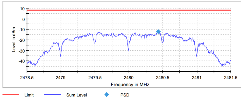
Figure 7.6.2-4: 2480MHz PSD Plot
