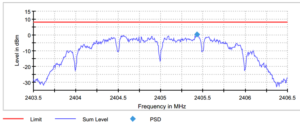
Figure 7.6.2-1: 2405MHz PSD Plot
