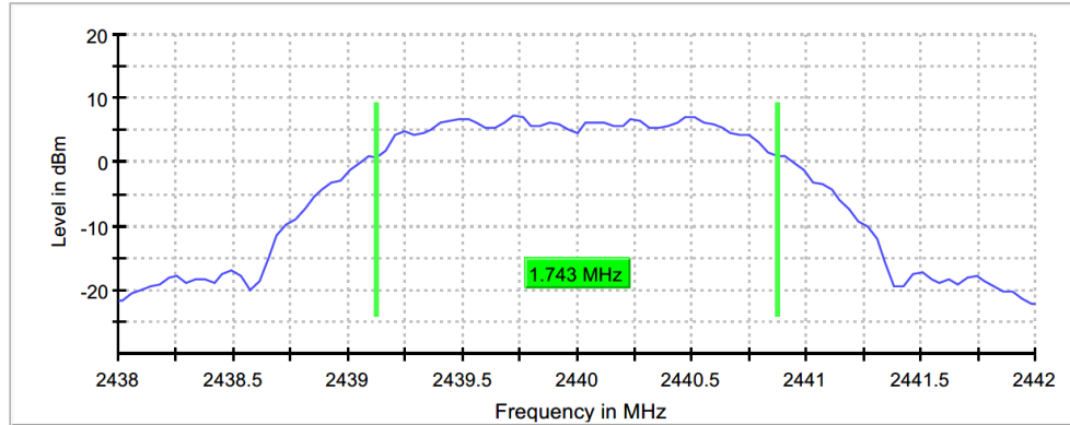
Figure 7.3.2-2: 2440MHz - 6dB BW
