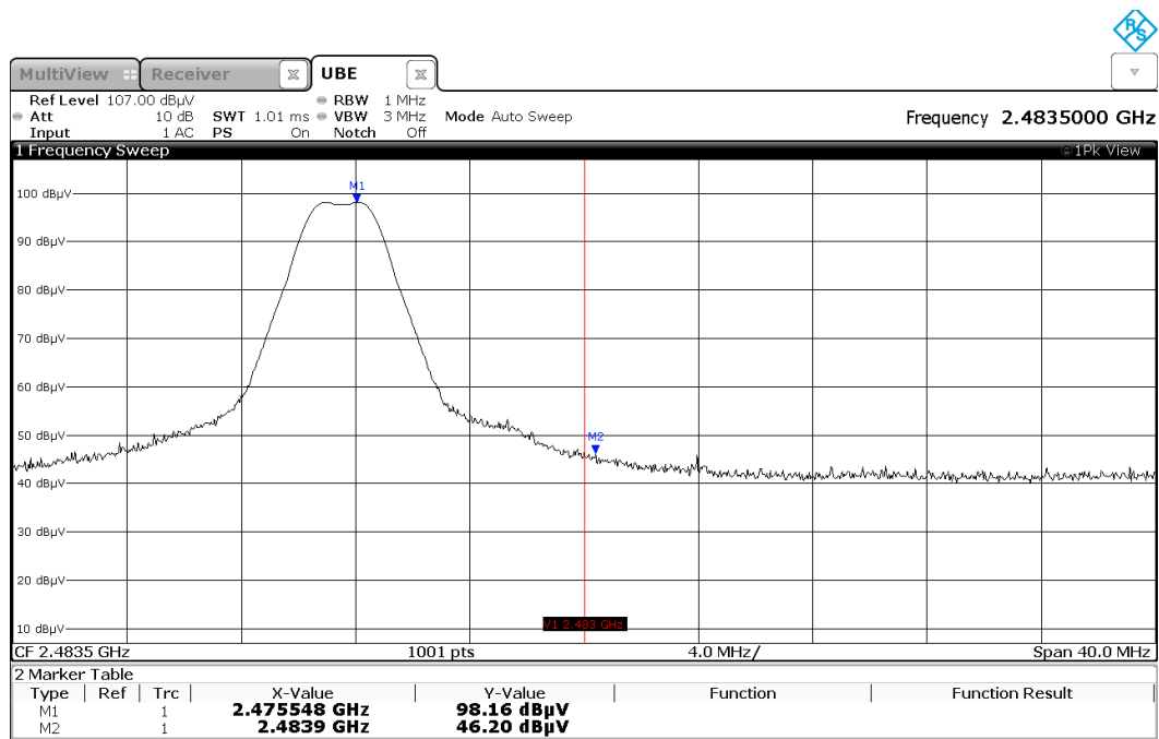
Figure A-8: Restricted Band Edge High – 2475MHz
