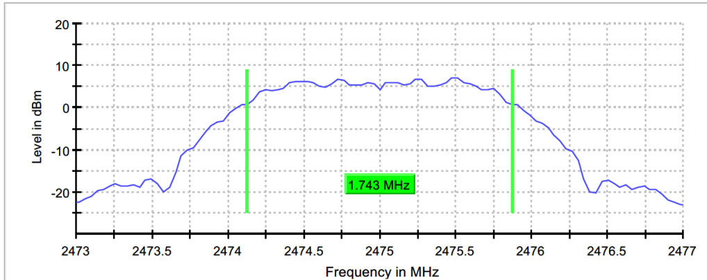
Figure 7.3.2-3: 2475MHz - 6dB BW
