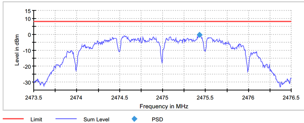
Figure 7.6.2-3: 2475MHz PSD Plot
