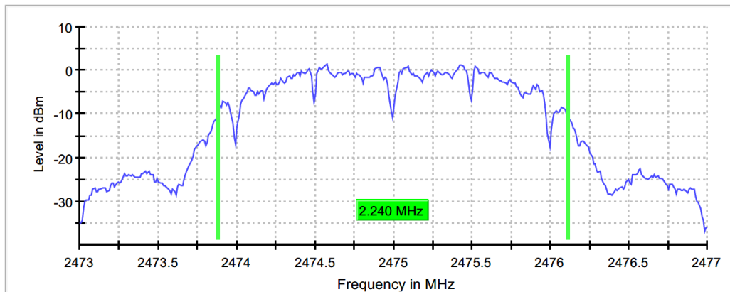
Figure 7.3.2-7: 2475MHz - 99% OBW
