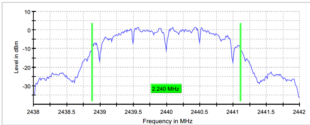
Figure 7.3.2-6: 2440MHz - 99% OBW
