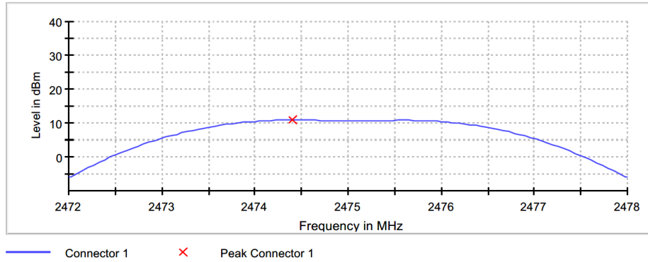
Figure 7.4.2-3: 2475MHz Plot
