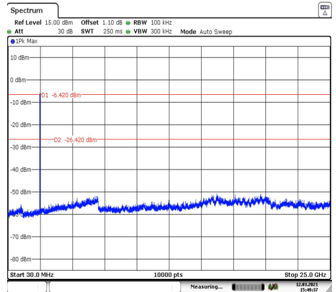
Figure 7.5.1.2-4: HCH (2480MHz) – 30MHz–25GHz
