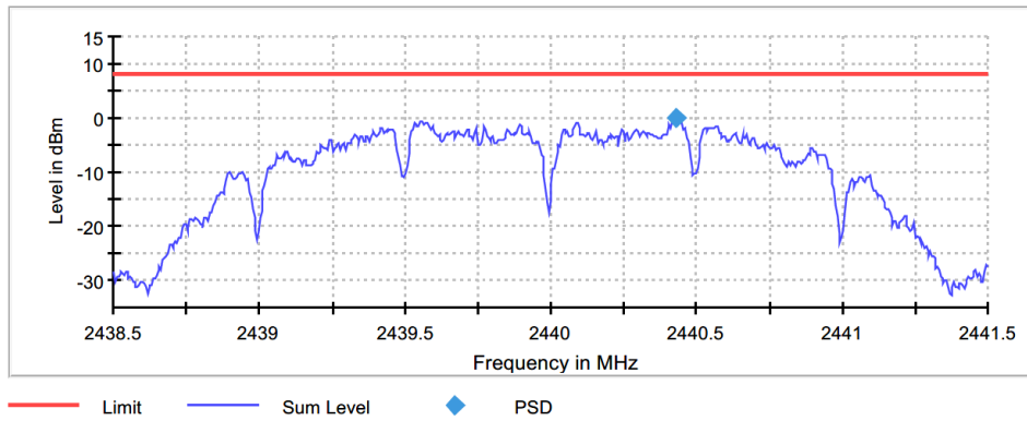
Figure 7.6.2-2: 2440MHz PSD Plot
