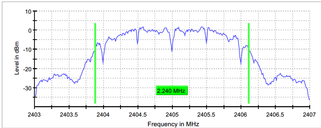
Figure 7.3.2-5: 2405MHz - 99% OBW
