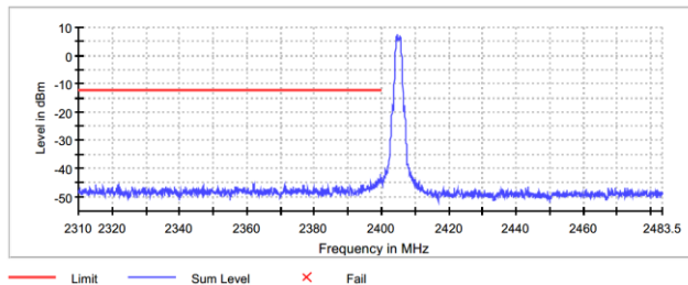
Figure 7.5.1.2-5: Lower Band-edge
