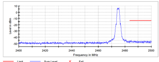
Figure 7.5.1.2-6: Upper Band-edge (2475MHz)
