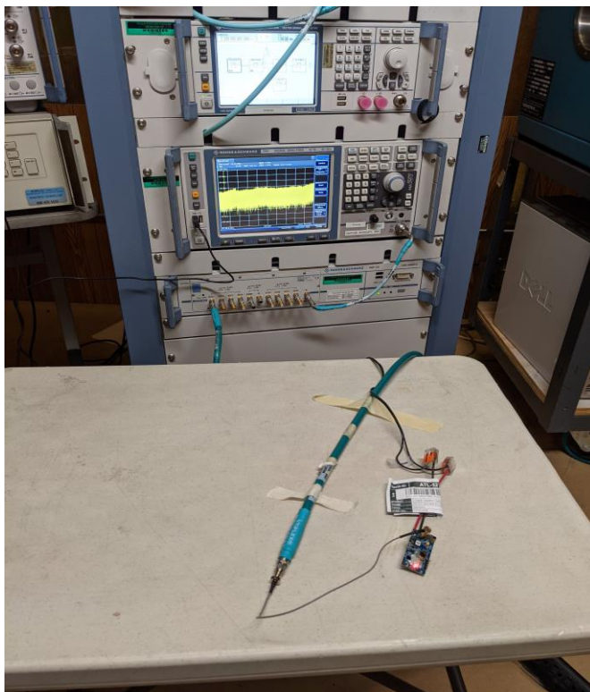
Figure 1: Equipment Under Test – Antenna Port Conducted Measurements
