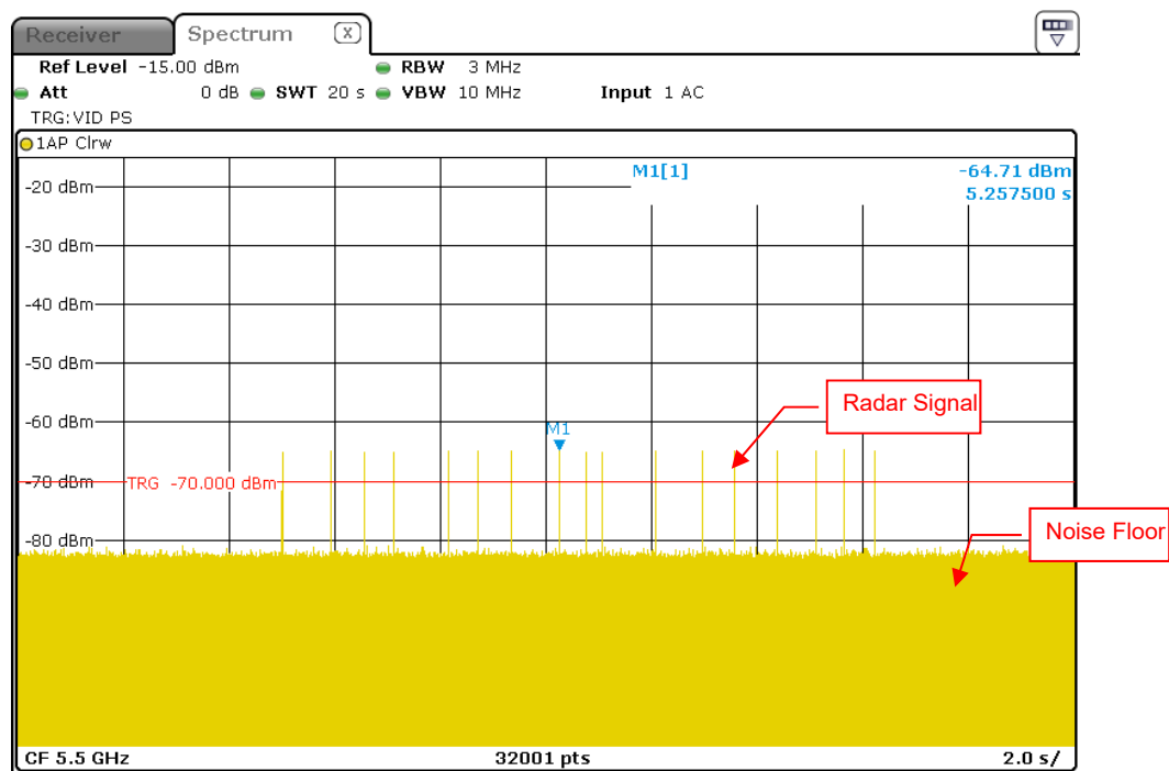
Radar Signal 5
