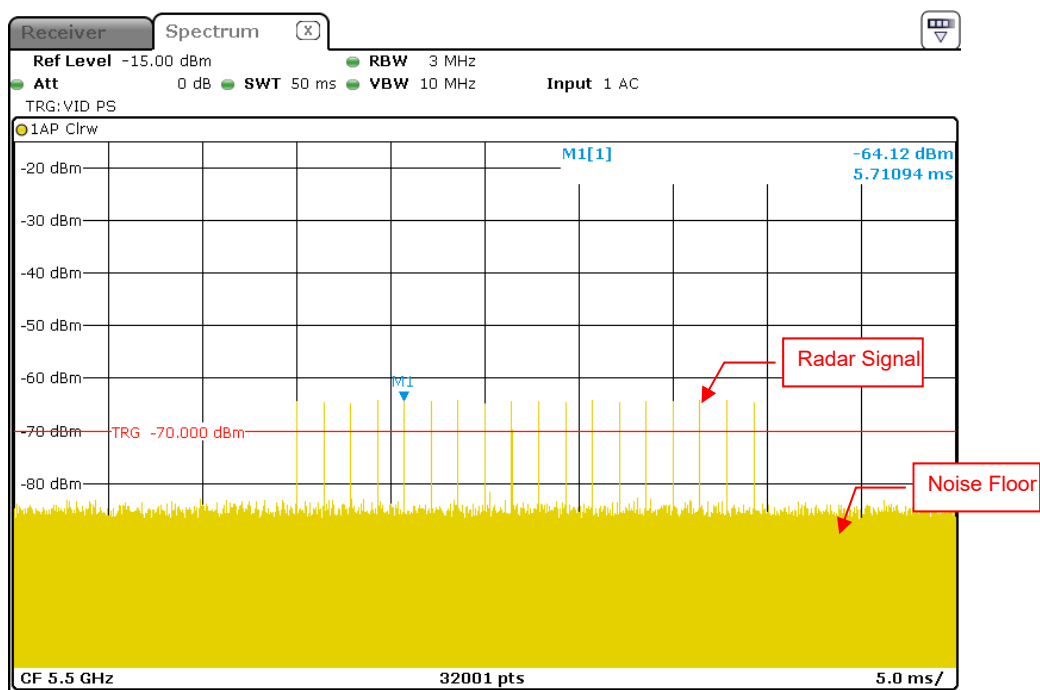
Radar Signal 0
