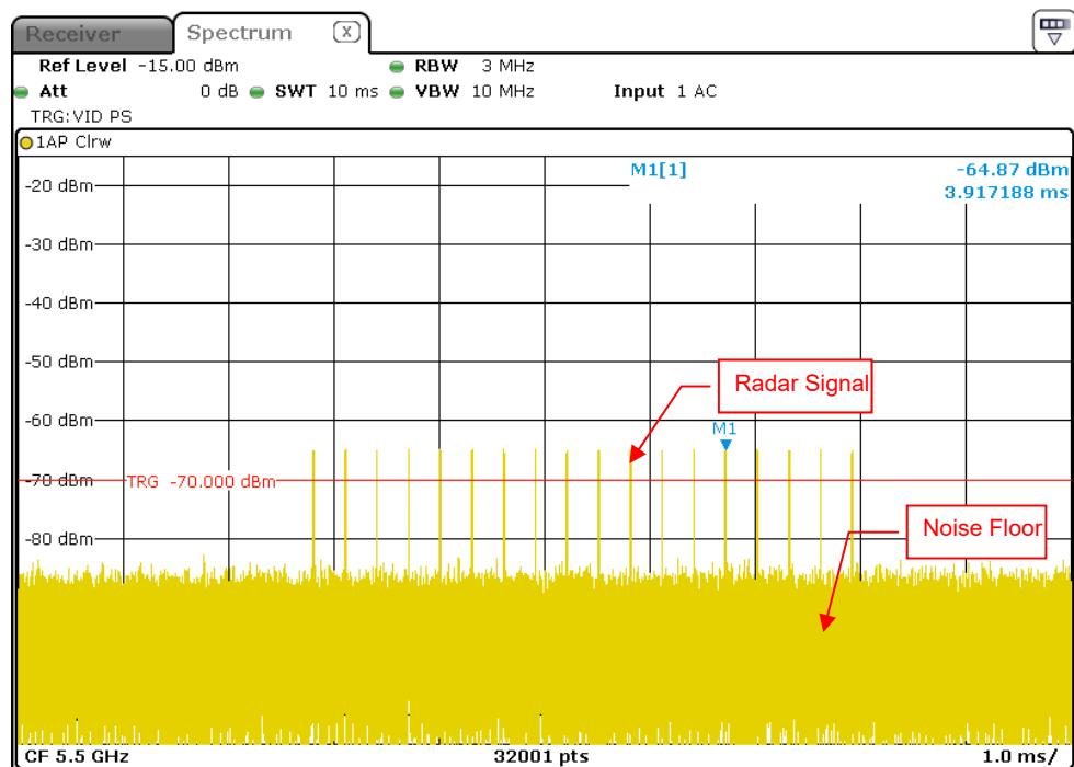
Radar Signal 3
