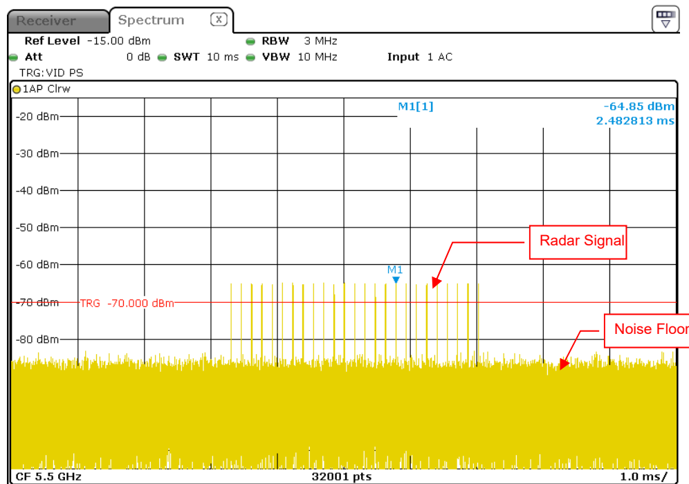
Radar Signal 2
