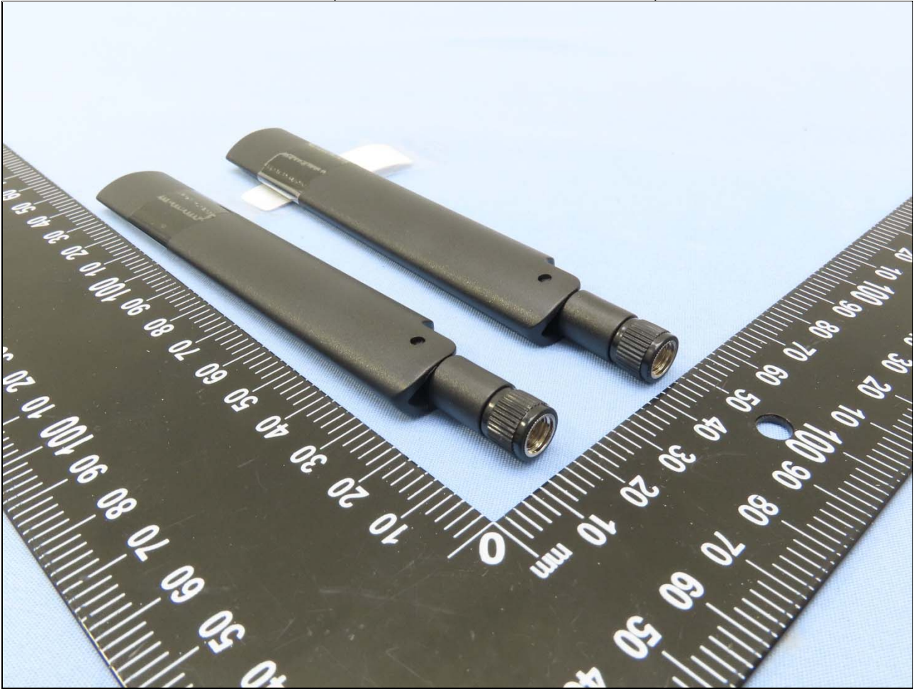
Antenna (Brand: AWAN, Model: A8PEE-100007)
