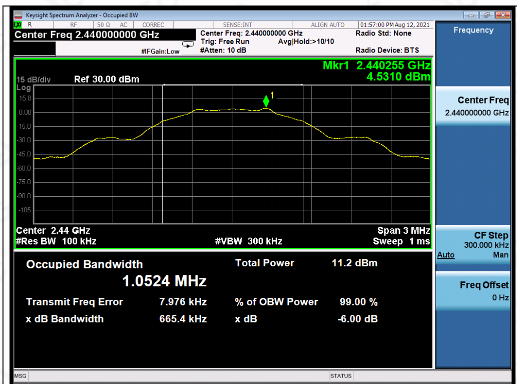
Test_Graph_LE1M_ANT1_2440_1Mbps_DTSBW
