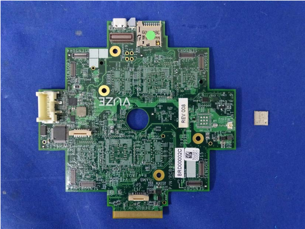
(16) EUT Photo (WiFi Module)
