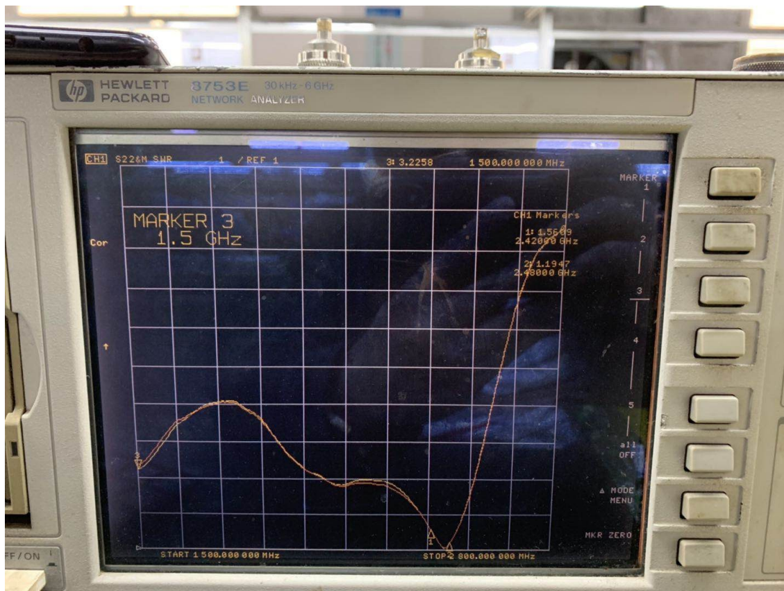
Standing wave ratio curve of BT antenna
