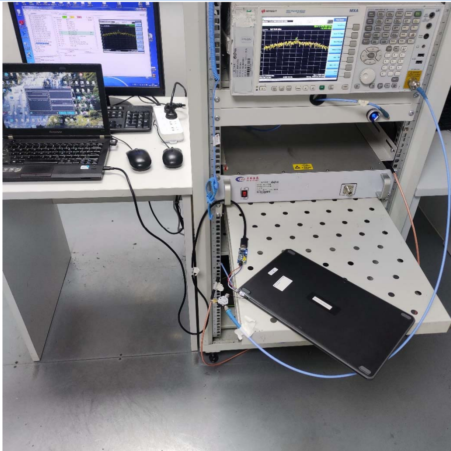
Conducted Test-BLE
