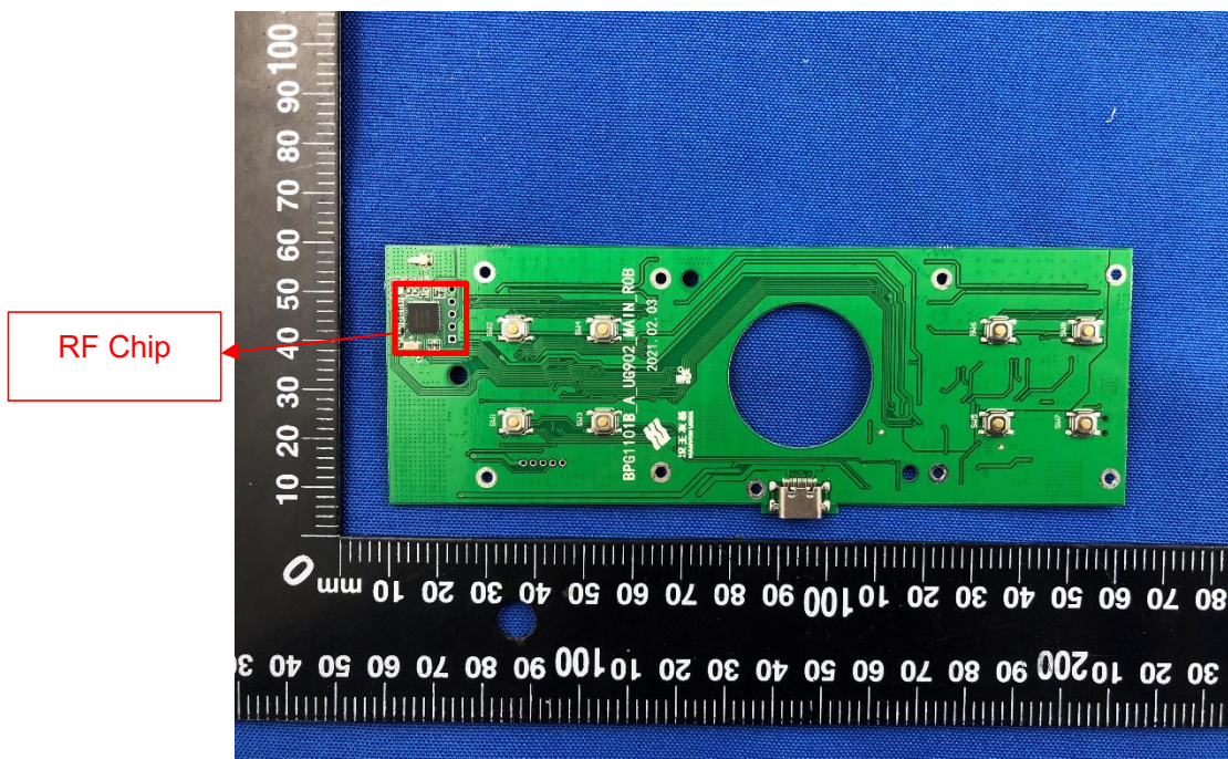
MAIN BOARD REAR VIEW
