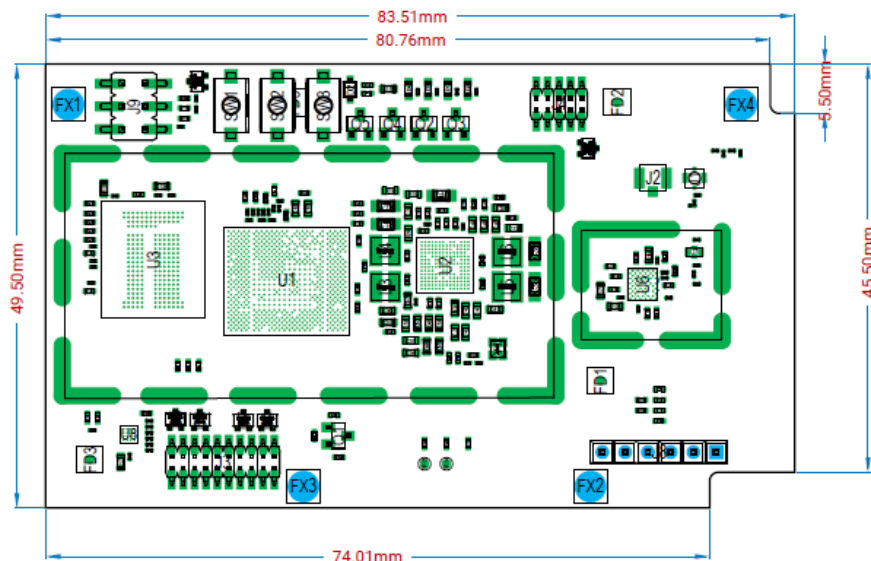
Figure 2. Mechanical Description.
