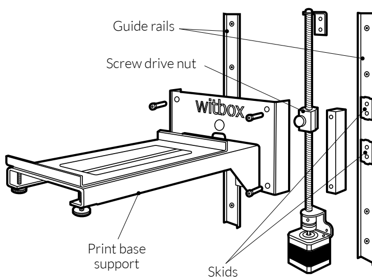
Figure 5.7 Constituent parts of the Z unit
