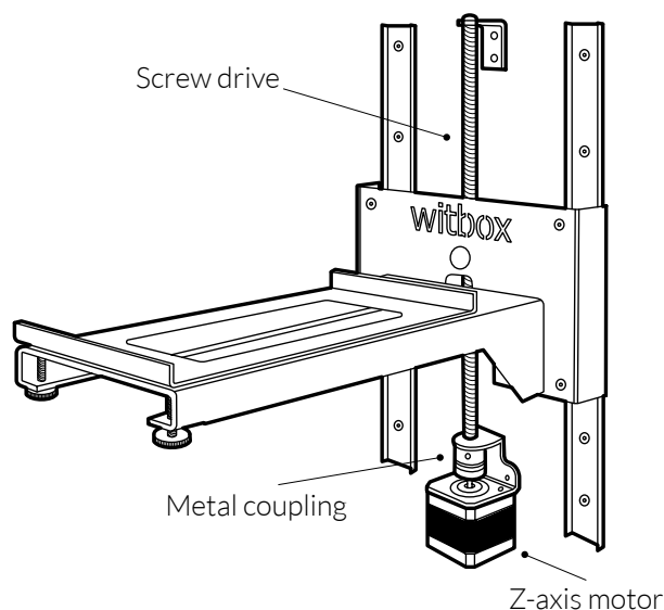
Figure 5.6 Z unit
