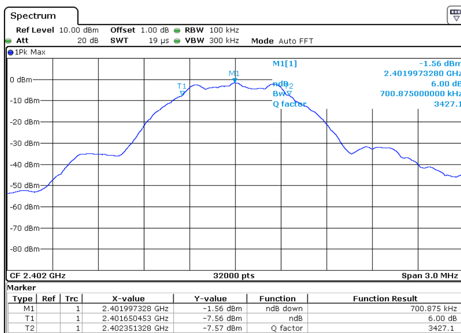
(1Mbps) The Low Channel 00: 2402 MHz
